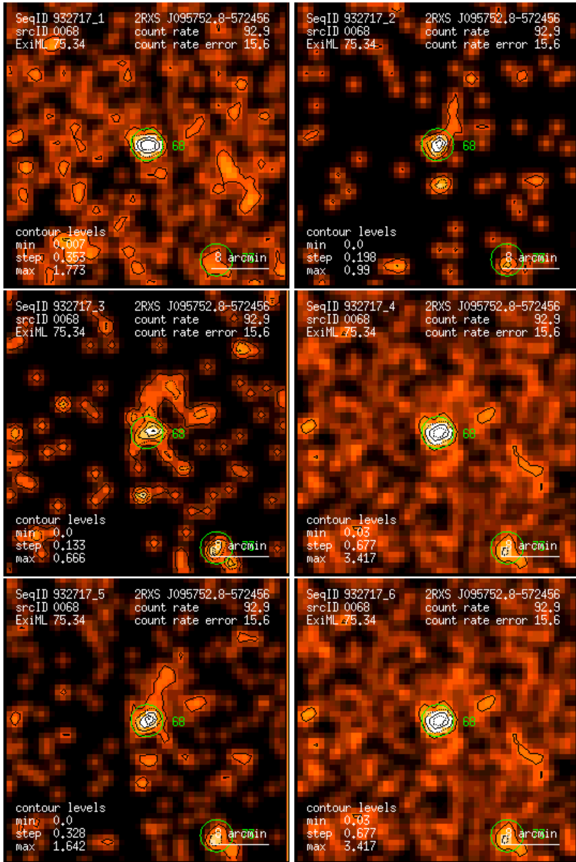
Figure 68: RASS 932717: detection 0068: band rate images, Gaussian filter: (1) PSPC channels 11 – 41, (2) 52 – 90, (3) 91 – 201, (4) 11 – 235, (5) 52 – 201, (6) 11 – 201. Broad band rates in counts/ks. Band rate contour levels in counts/ks/arcmin 2 .
