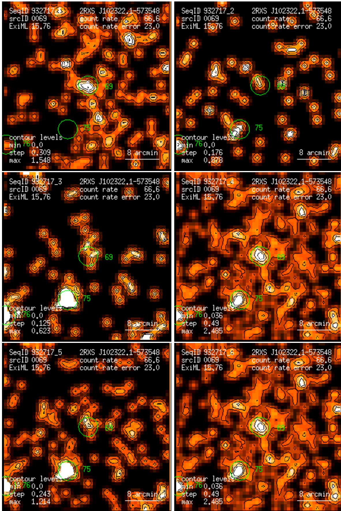
Figure 69: RASS 932717: detection 0069: band rate images, Gaussian filter: (1) PSPC channels 11 – 41, (2) 52 – 90, (3) 91 – 201, (4) 11 – 235, (5) 52 – 201, (6) 11 – 201. Broad band rates in counts/ks. Band rate contour levels in counts/ks/arcmin 2 .
