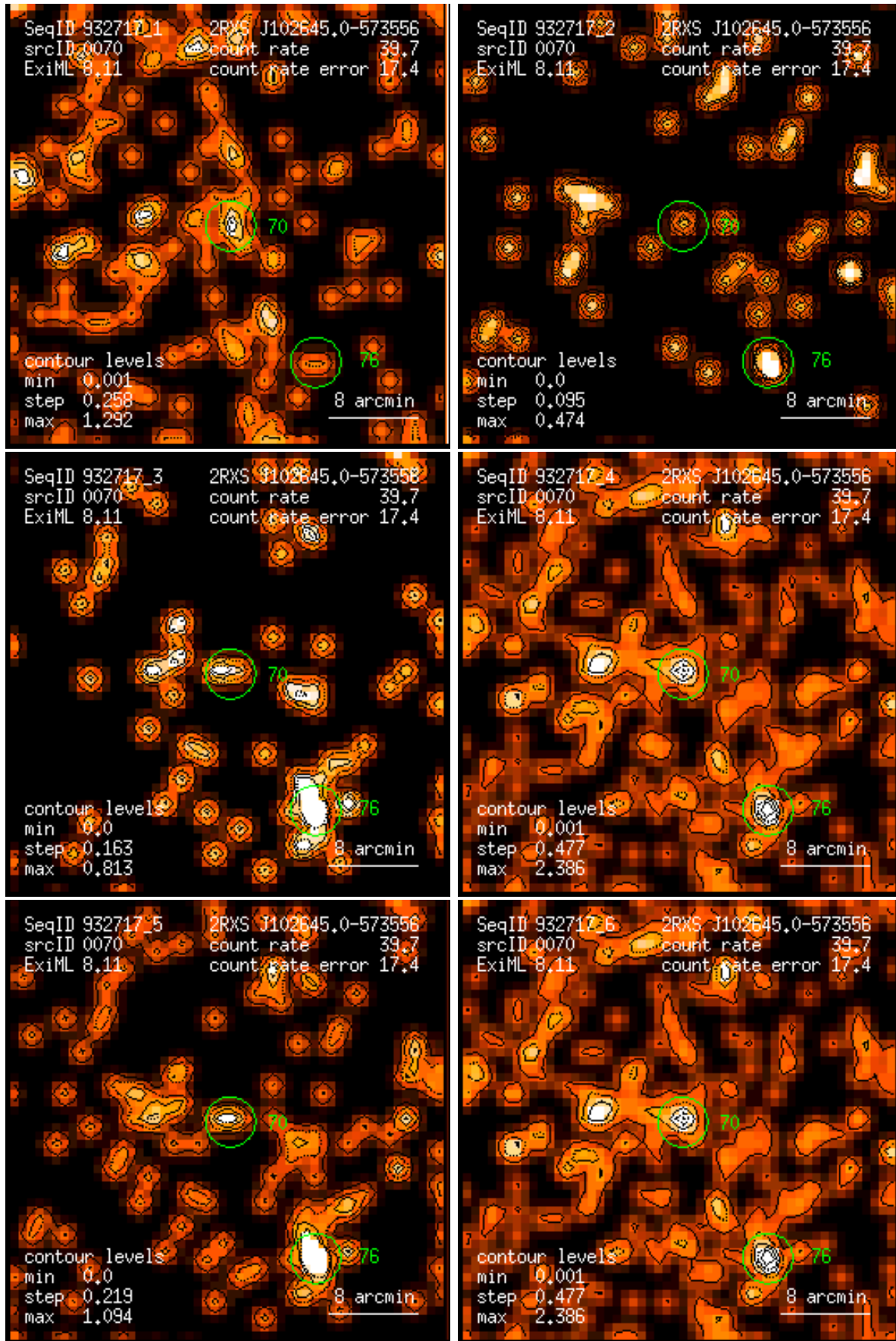
Figure 70: RASS 932717: detection 0070: band rate images, Gaussian filter: (1) PSPC channels 11 – 41, (2) 52 – 90, (3) 91 – 201, (4) 11 – 235, (5) 52 – 201, (6) 11 – 201. Broad band rates in counts/ks. Band rate contour levels in counts/ks/arcmin 2 .
