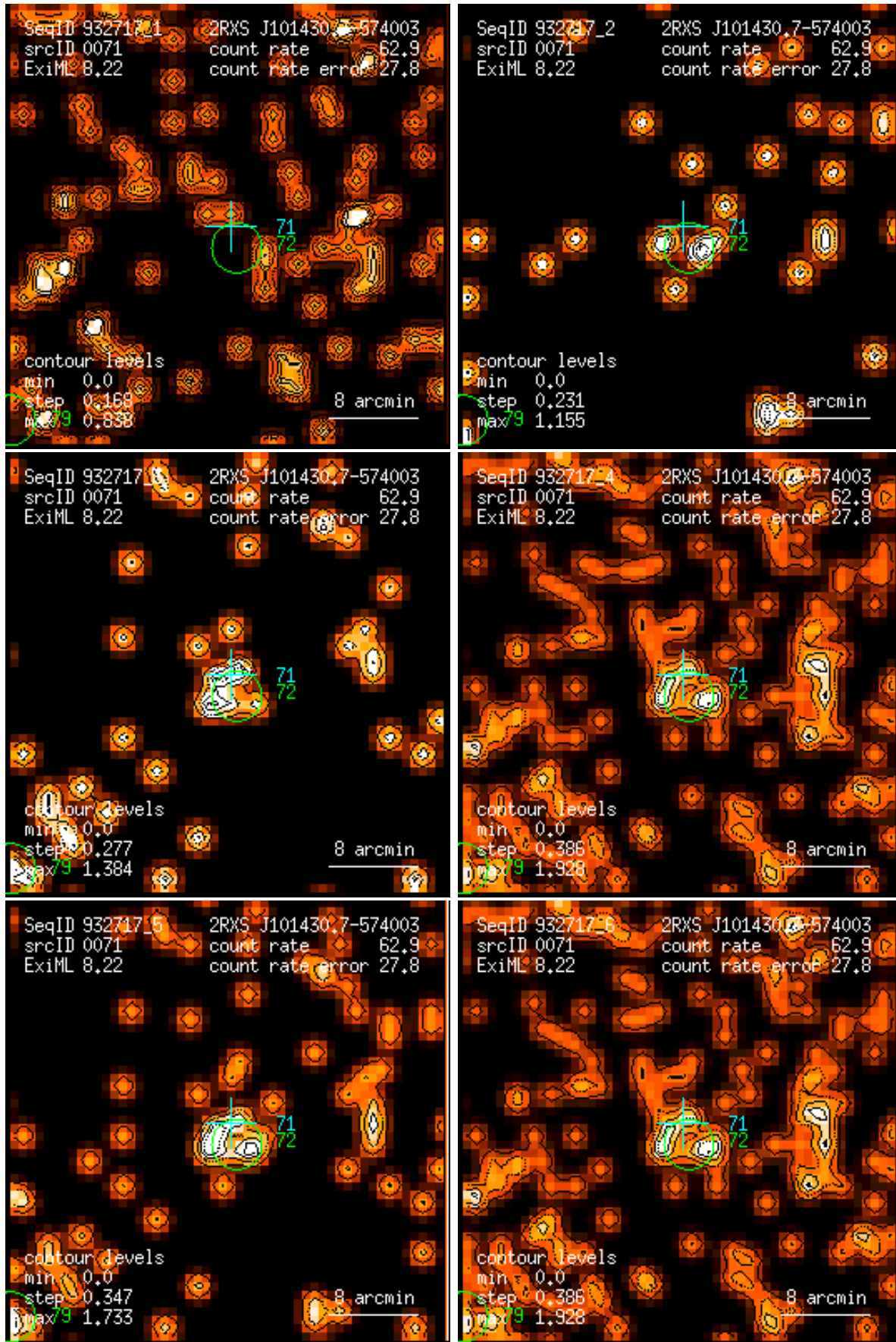
Figure 71: RASS 932717: detection 0071: band rate images, Gaussian filter: (1) PSPC channels 11 – 41, (2) 52 – 90, (3) 91 – 201, (4) 11 – 235, (5) 52 – 201, (6) 11 – 201. Broad band rates in counts/ks. Band rate contour levels in counts/ks/arcmin 2 .
