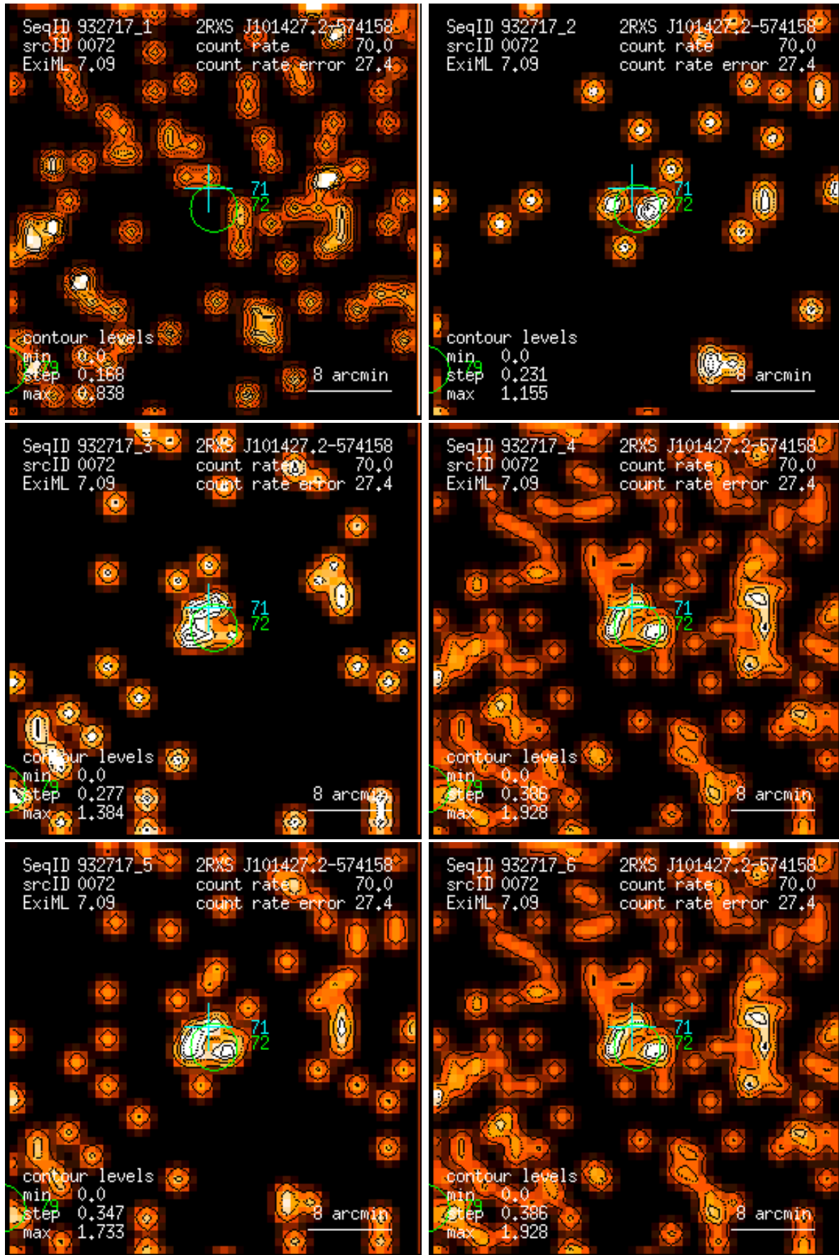
Figure 72: RASS 932717: detection 0072: band rate images, Gaussian filter: (1) PSPC channels 11 – 41, (2) 52 – 90, (3) 91 – 201, (4) 11 – 235, (5) 52 – 201, (6) 11 – 201. Broad band rates in counts/ks. Band rate contour levels in counts/ks/arcmin 2 .
