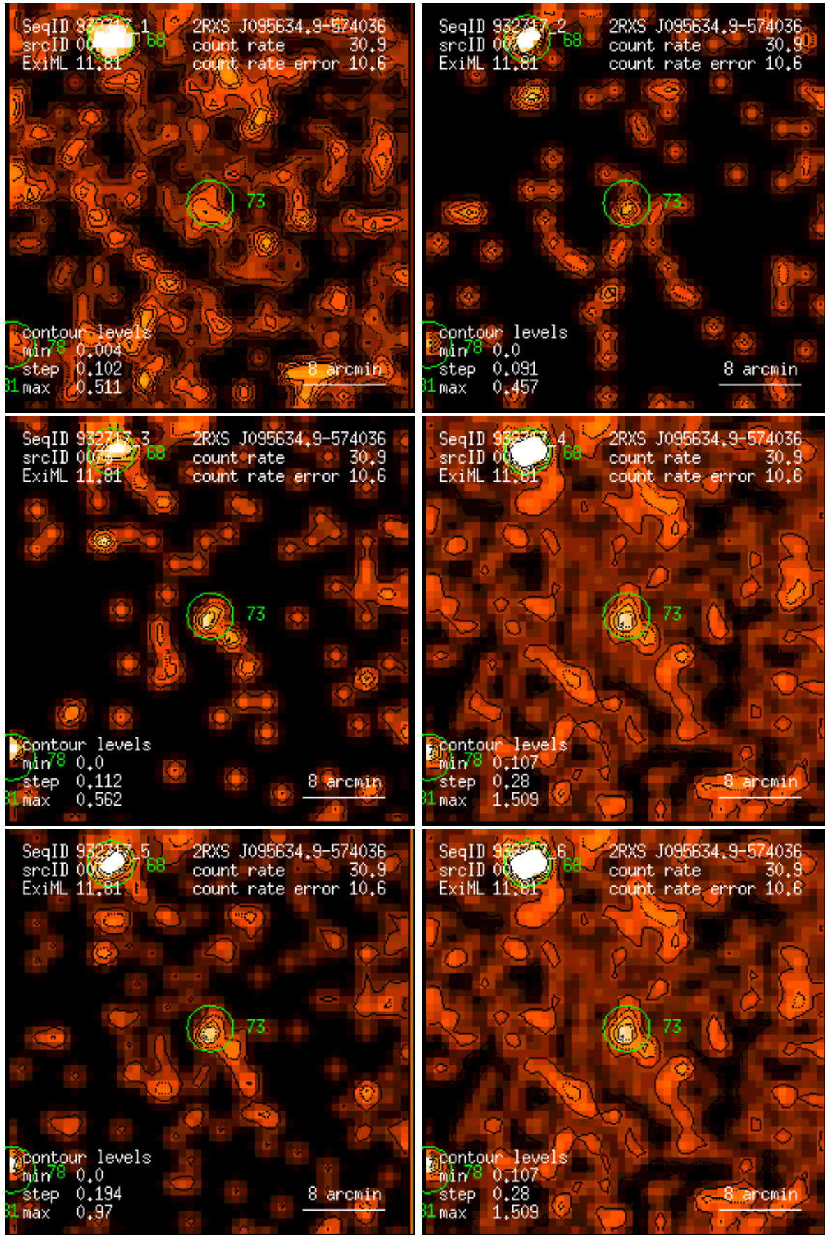
Figure 73: RASS 932717: detection 0073: band rate images, Gaussian filter: (1) PSPC channels 11 – 41, (2) 52 – 90, (3) 91 – 201, (4) 11 – 235, (5) 52 – 201, (6) 11 – 201. Broad band rates in counts/ks. Band rate contour levels in counts/ks/arcmin 2 .
