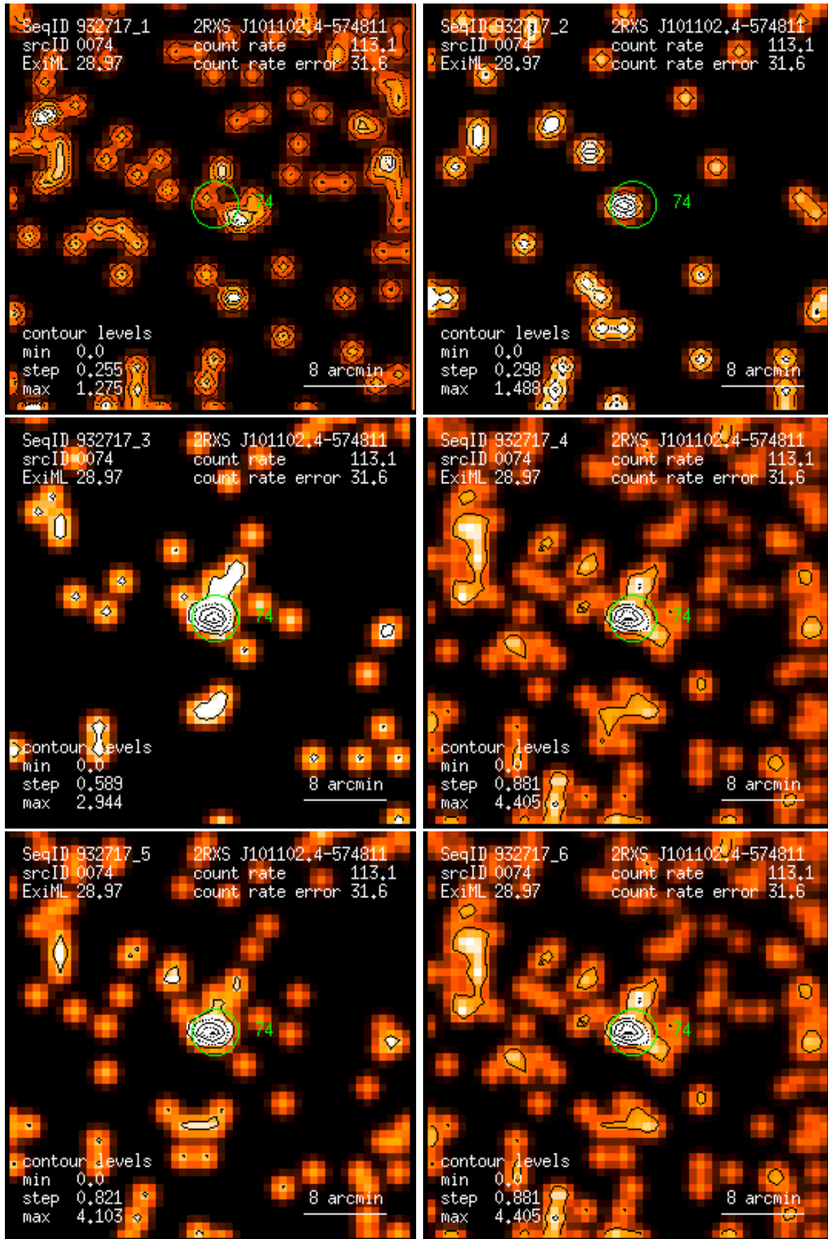
Figure 74: RASS 932717: detection 0074: band rate images, Gaussian filter: (1) PSPC channels 11 – 41, (2) 52 – 90, (3) 91 – 201, (4) 11 – 235, (5) 52 – 201, (6) 11 – 201. Broad band rates in counts/ks. Band rate contour levels in counts/ks/arcmin 2 .
