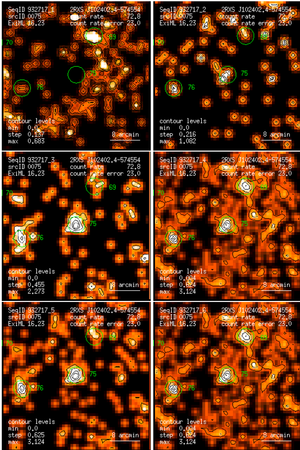
Figure 75: RASS 932717: detection 0075: band rate images, Gaussian filter: (1) PSPC channels 11 – 41, (2) 52 – 90, (3) 91 – 201, (4) 11 – 235, (5) 52 – 201, (6) 11 – 201. Broad band rates in counts/ks. Band rate contour levels in counts/ks/arcmin 2 .
