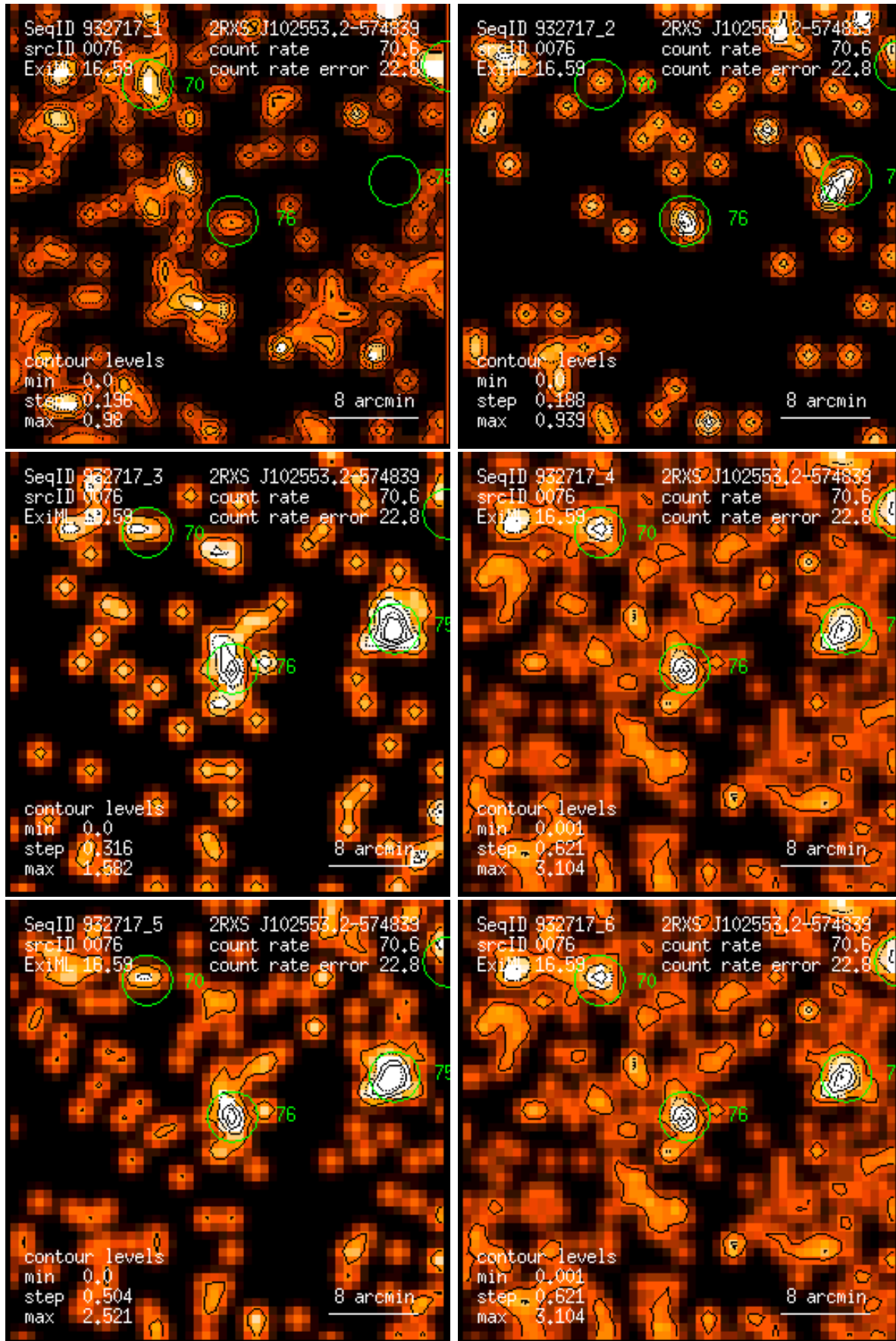
Figure 76: RASS 932717: detection 0076: band rate images, Gaussian filter: (1) PSPC channels 11 – 41, (2) 52 – 90, (3) 91 – 201, (4) 11 – 235, (5) 52 – 201, (6) 11 – 201. Broad band rates in counts/ks. Band rate contour levels in counts/ks/arcmin 2 .
