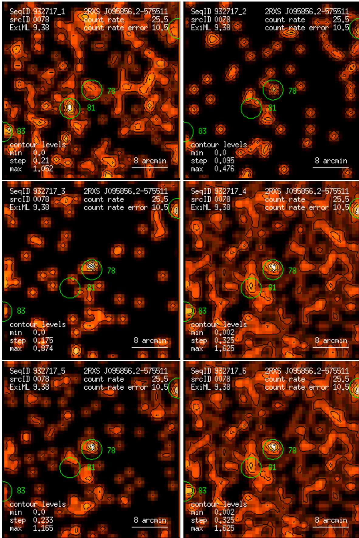
Figure 78: RASS 932717: detection 0078: band rate images, Gaussian filter: (1) PSPP channels 11 – 41, (2) 52 – 90, (3) 91 – 201, (4) 11 – 235, (5) 52 – 201, (6) 11 – 201. Broad band rates in counts/ks. Band rate contour levels in counts/ks/arcmin 2 .
