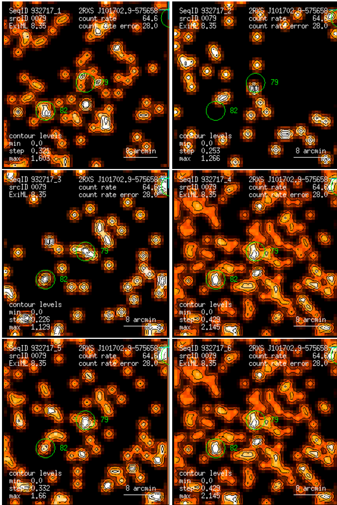
Figure 79: RASS 932717: detection 0079: band rate images, Gaussian filter: (1) PSPC channels 11 – 41, (2) 52 – 90, (3) 91 – 201, (4) 11 – 235, (5) 52 – 201, (6) 11 – 201. Broad band rates in counts/ks. Band rate contour levels in counts/ks/arcmin 2 .
