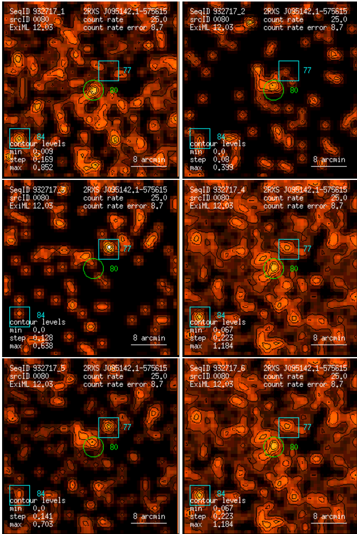
Figure 80: RASS 932717: detection 0080: band rate images, Gaussian filter: (1) PSPC channels 11 – 41, (2) 52 – 90, (3) 91 – 201, (4) 11 – 235, (5) 52 – 201, (6) 11 – 201. Broad band rates in counts/ks. Band rate contour levels in counts/ks/arcmin 2 .
