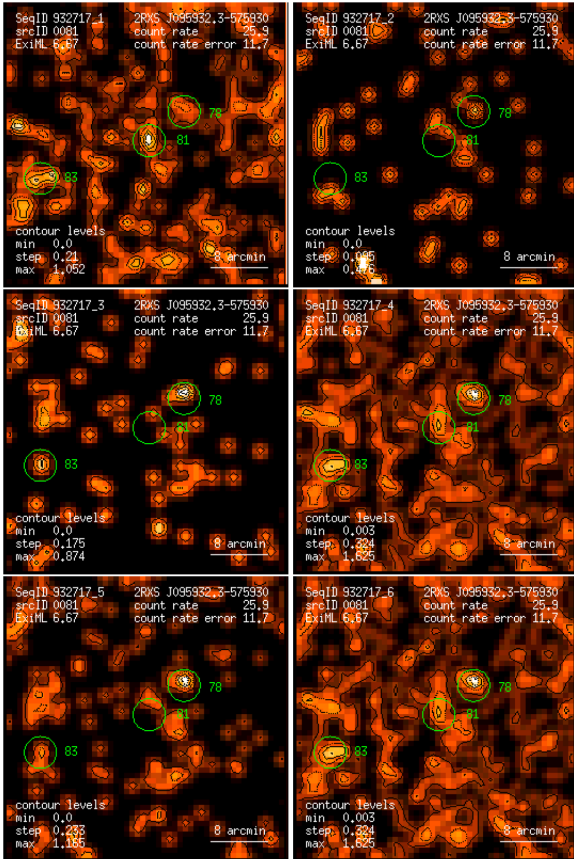
Figure 81: RASS 932717: detection 0081: band rate images, Gaussian filter: (1) PSPC channels 11 – 41, (2) 52 – 90, (3) 91 – 201, (4) 11 – 235, (5) 52 – 201, (6) 11 – 201. Broad band rates in counts/ks. Band rate contour levels in counts/ks/arcmin 2 .
