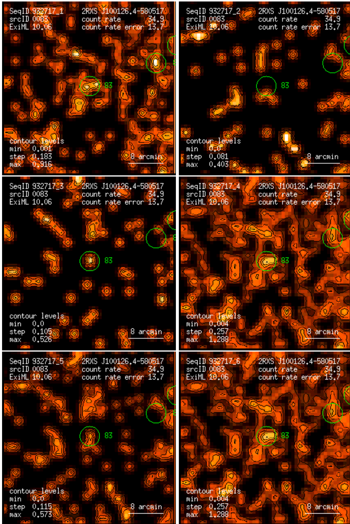
Figure 83: RASS 932717: detection 0083: band rate images, Gaussian filter: (1) PSPC channels 11 – 41, (2) 52 – 90, (3) 91 – 201, (4) 11 – 235, (5) 52 – 201, (6) 11 – 201. Broad band rates in counts/ks. Band rate contour levels in counts/ks/arcmin 2 .
