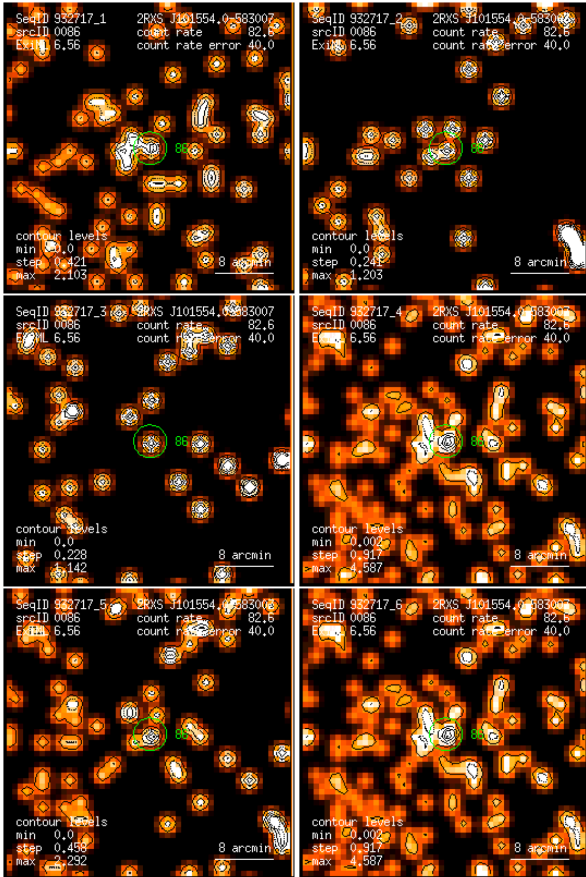
Figure 86: RASS 932717: detection 0086: band rate images, Gaussian filter: (1) PSPC channels 11 – 41, (2) 52 – 90, (3) 91 – 201, (4) 11 – 235, (5) 52 – 201, (6) 11 – 201. Broad band rates in counts/ks. Band rate contour levels in counts/ks/arcmin 2 .
