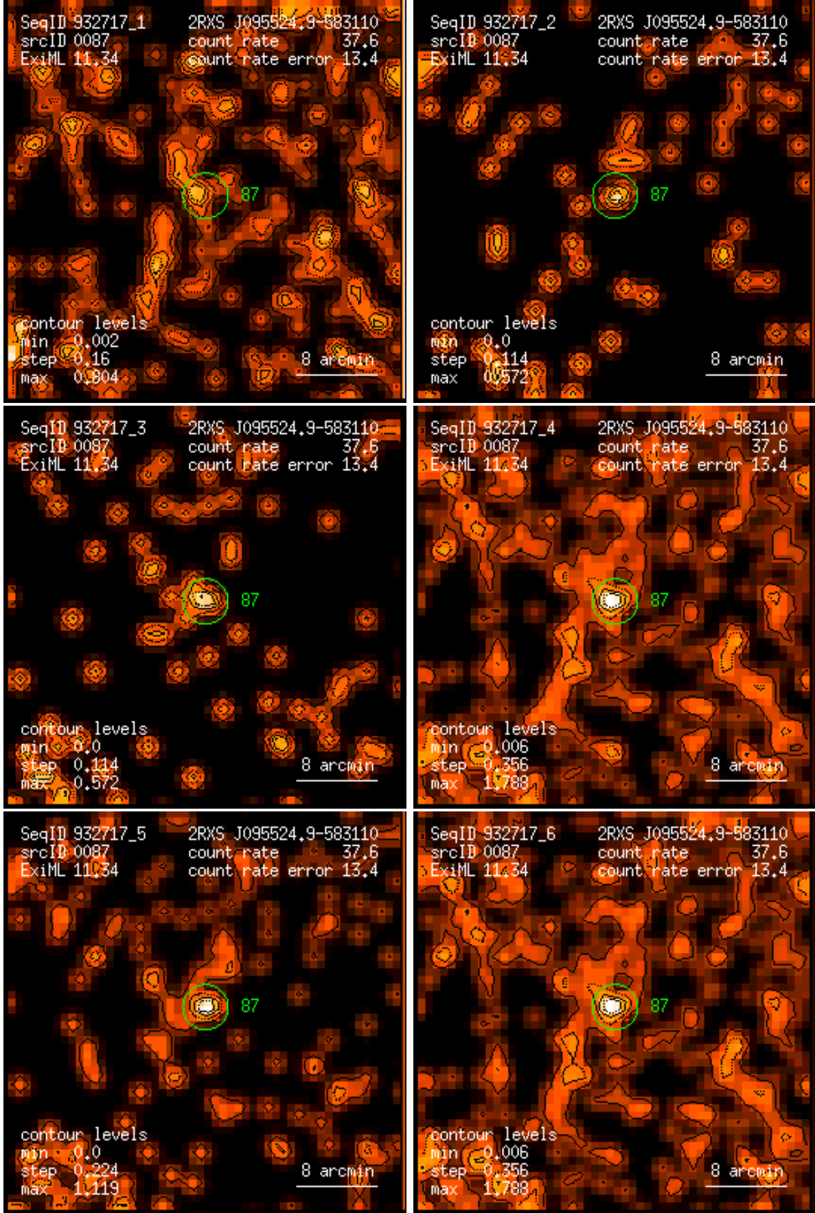
Figure 87: RASS 932717: detection 0087: band rate images, Gaussian filter: (1) PSPC channels 11 – 41, (2) 52 – 90, (3) 91 – 201, (4) 11 – 235, (5) 52 – 201, (6) 11 – 201. Broad band rates in counts/ks. Band rate contour levels in counts/ks/arcmin 2 .
