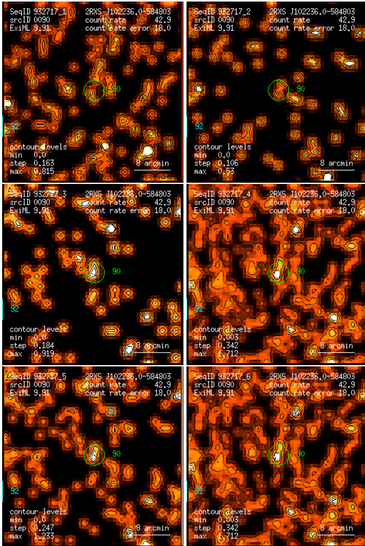
Figure 90: RASS 932717: detection 0090: band rate images, Gaussian filter: (1) PSPC channels 11 – 41, (2) 52 – 90, (3) 91 – 201, (4) 11 – 235, (5) 52 – 201, (6) 11 – 201. Broad band rates in counts/ks. Band rate contour levels in counts/ks/arcmin 2 .
