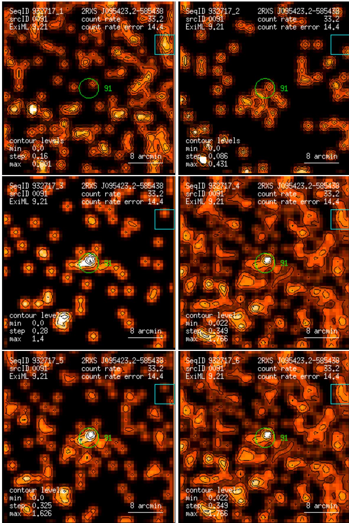
Figure 91: RASS 932717: detection 0091: band rate images, Gaussian filter: (1) PSPC channels 11 – 41, (2) 52 – 90, (3) 91 – 201, (4) 11 – 235, (5) 52 – 201, (6) 11 – 201. Broad band rates in counts/ks. Band rate contour levels in counts/ks/arcmin 2 .
