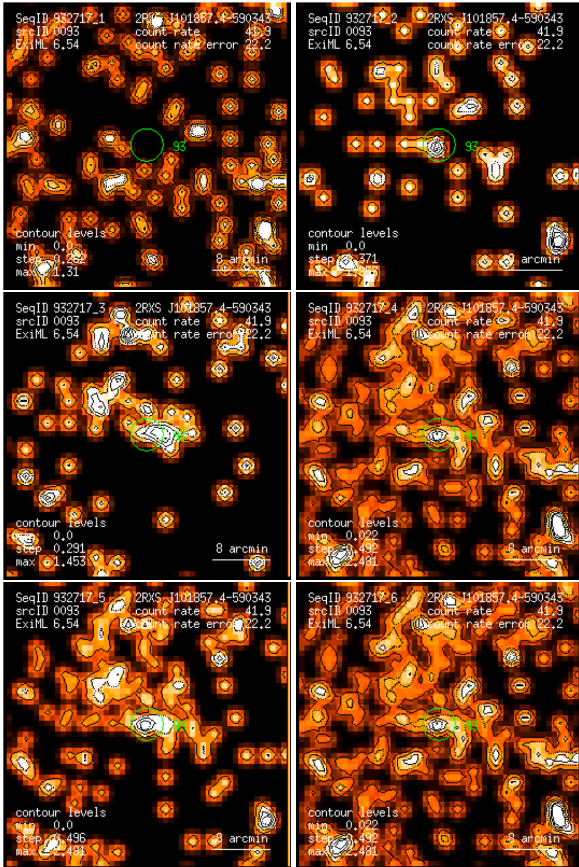
Figure 93: RASS 932717: detection 0093: band rate images, Gaussian filter: (1) PSPC channels 11 – 41, (2) 52 – 90, (3) 91 – 201, (4) 11 – 235, (5) 52 – 201, (6) 11 – 201. Broad band rates in counts/ks. Band rate contour levels in counts/ks/arcmin 2 .
