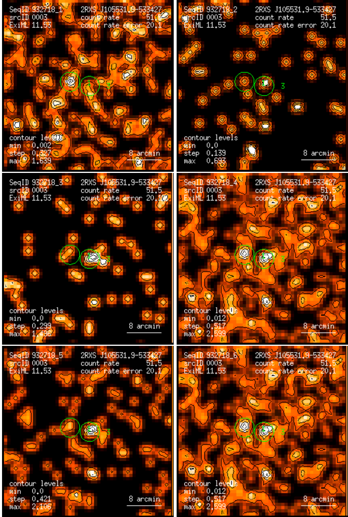
Figure 3: RASS 932718: detection 0003: band rate images, Gaussian filter: (1) PSPC channels 11 – 41, (2) 52 – 90, (3) 91 – 201, (4) 11 – 235, (5) 52 – 201, (6) 11 – 201. Broad band rates in counts/ks. Band rate contour levels in counts/ks/arcmin 2 .
