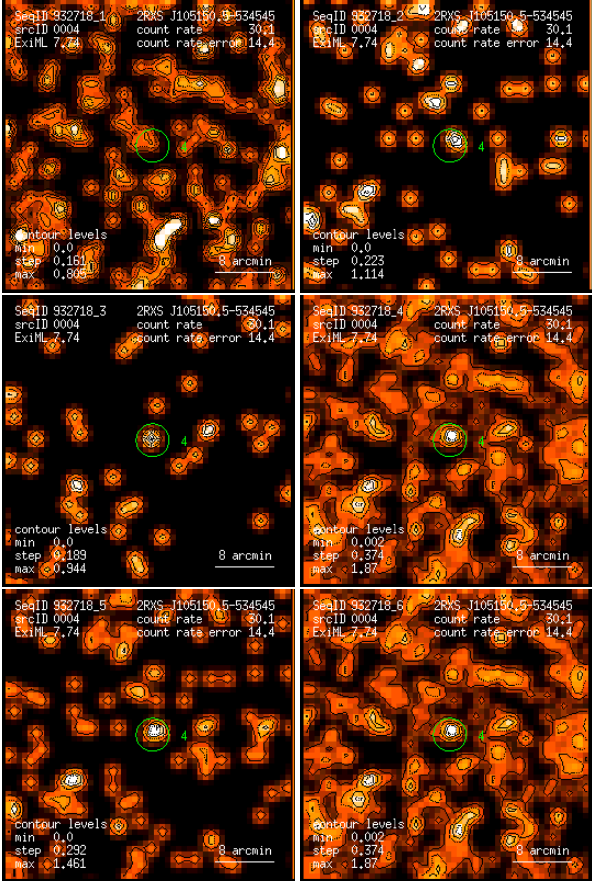
Figure 4: RASS 932718: detection 0004: band rate images, Gaussian filter: (1) PSPC channels 11 – 41, (2) 52 – 90, (3) 91 – 201, (4) 11 – 235, (5) 52 – 201, (6) 11 – 201. Broad band rates in counts/ks. Band rate contour levels in counts/ks/arcmin 2 .
