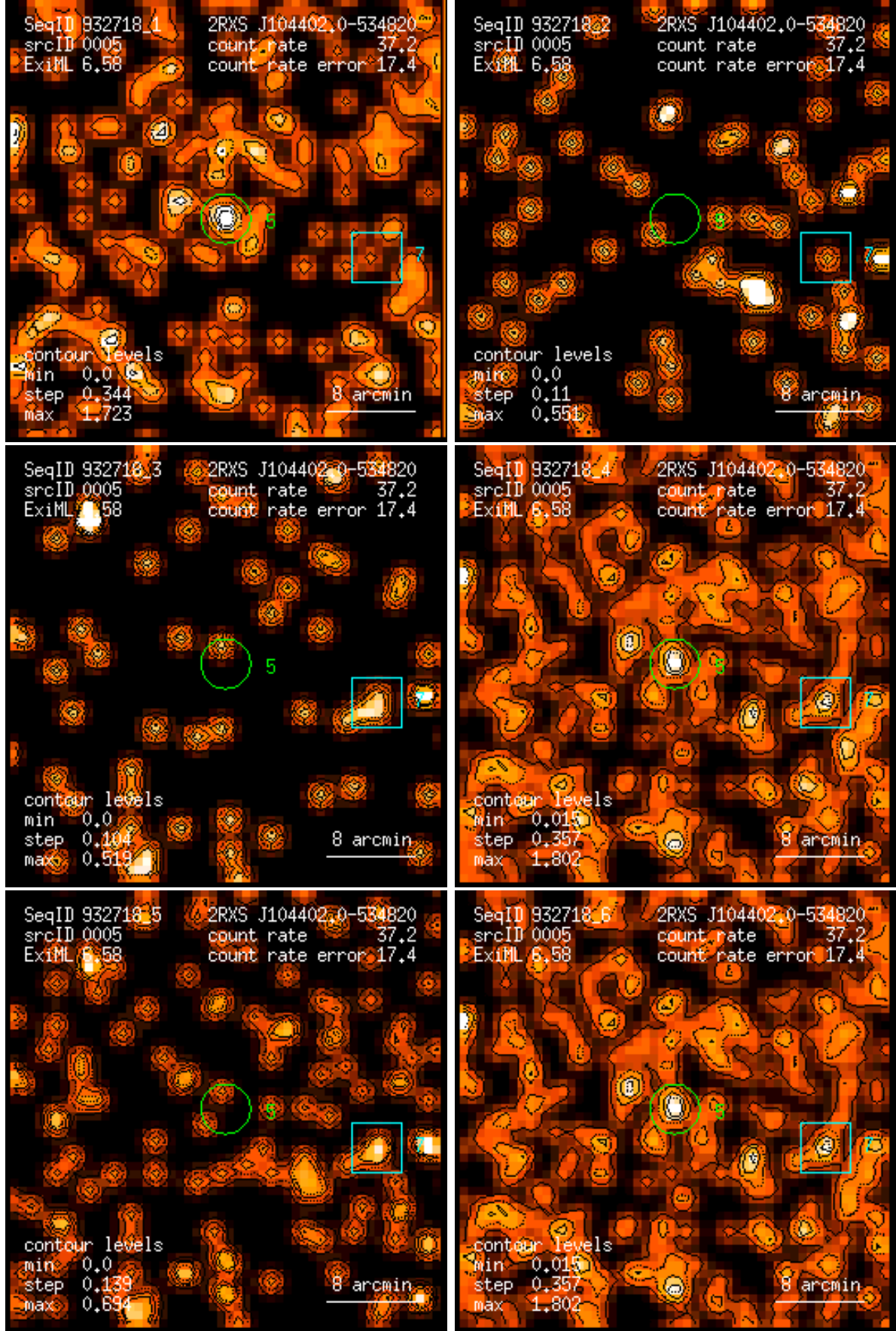
Figure 5: RASS 932718: detection 0005: band rate images, Gaussian filter: (1) PSPC channels 11 – 41, (2) 52 – 90, (3) 91 – 201, (4) 11 – 235, (5) 52 – 201, (6) 11 – 201. Broad band rates in counts/ks. Band rate contour levels in counts/ks/arcmin 2 .
