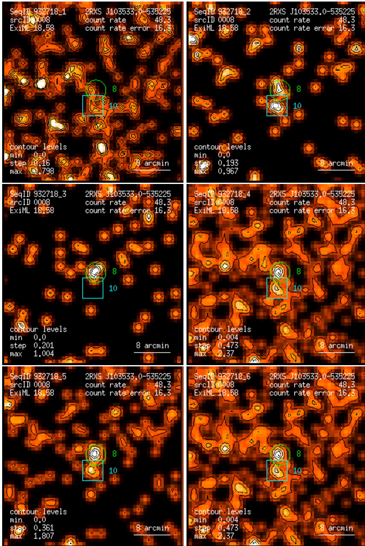
Figure 8: RASS 932718: detection 0008: band rate images, Gaussian filter: (1) PSPC channels 11 – 41, (2) 52 – 90, (3) 91 – 201, (4) 11 – 235, (5) 52 – 201, (6) 11 – 201. Broad band rates in counts/ks. Band rate contour levels in counts/ks/arcmin 2 .
