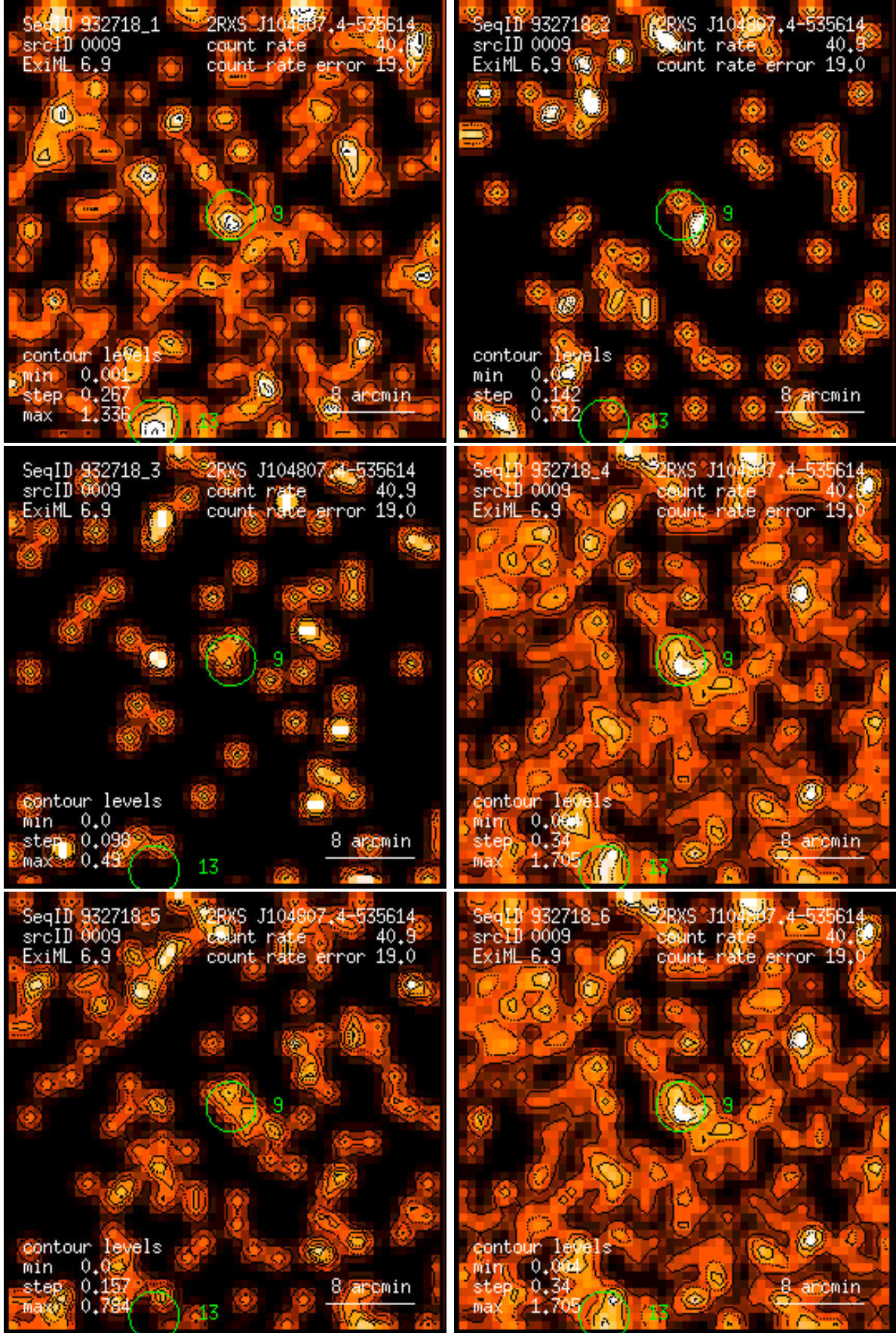
Figure 9: RASS 932718: detection 0009: band rate images, Gaussian filter: (1) PSPC channels 11 – 41, (2) 52 – 90, (3) 91 – 201, (4) 11 – 235, (5) 52 – 201, (6) 11 – 201. Broad band rates in counts/ks. Band rate contour levels in counts/ks/arcmin 2 .
