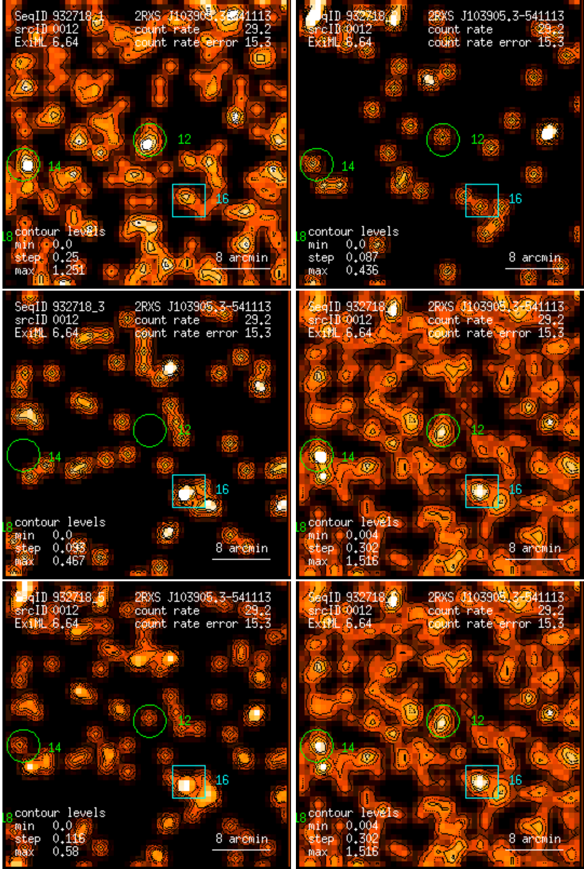
Figure 12: RASS 932718: detection 0012: band rate images, Gaussian filter: (1) PSPC channels 11 – 41, (2) 52 – 90, (3) 91 – 201, (4) 11 – 235, (5) 52 – 201, (6) 11 – 201. Broad band rates in counts/ks. Band rate contour levels in counts/ks/arcmin 2 .
