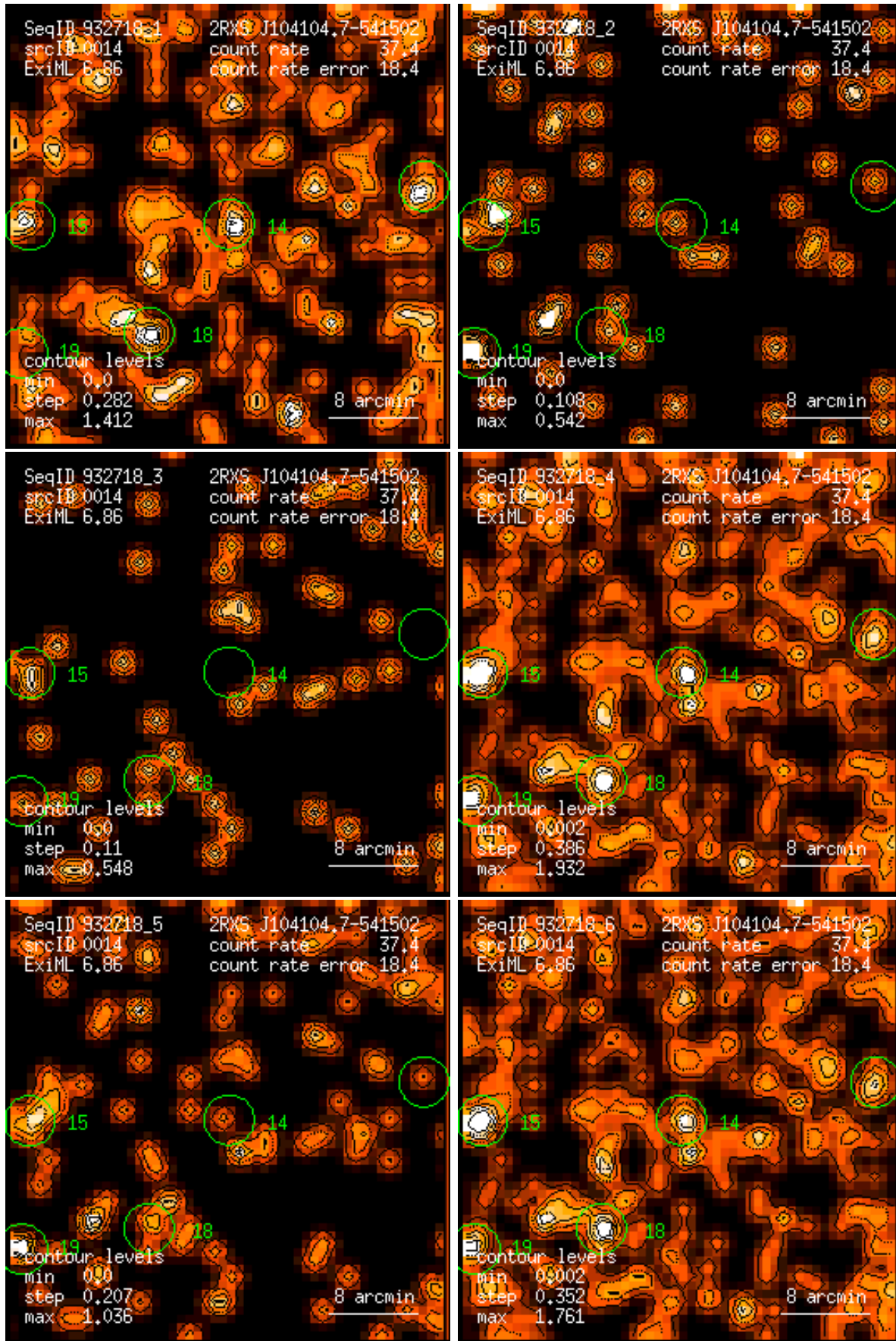
Figure 14: RASS 932718: detection 0014: band rate images, Gaussian filter: (1) PSPC channels 11 – 41, (2) 52 – 90, (3) 91 – 201, (4) 11 – 235, (5) 52 – 201, (6) 11 – 201. Broad band rates in counts/ks. Band rate contour levels in counts/ks/arcmin 2 .
