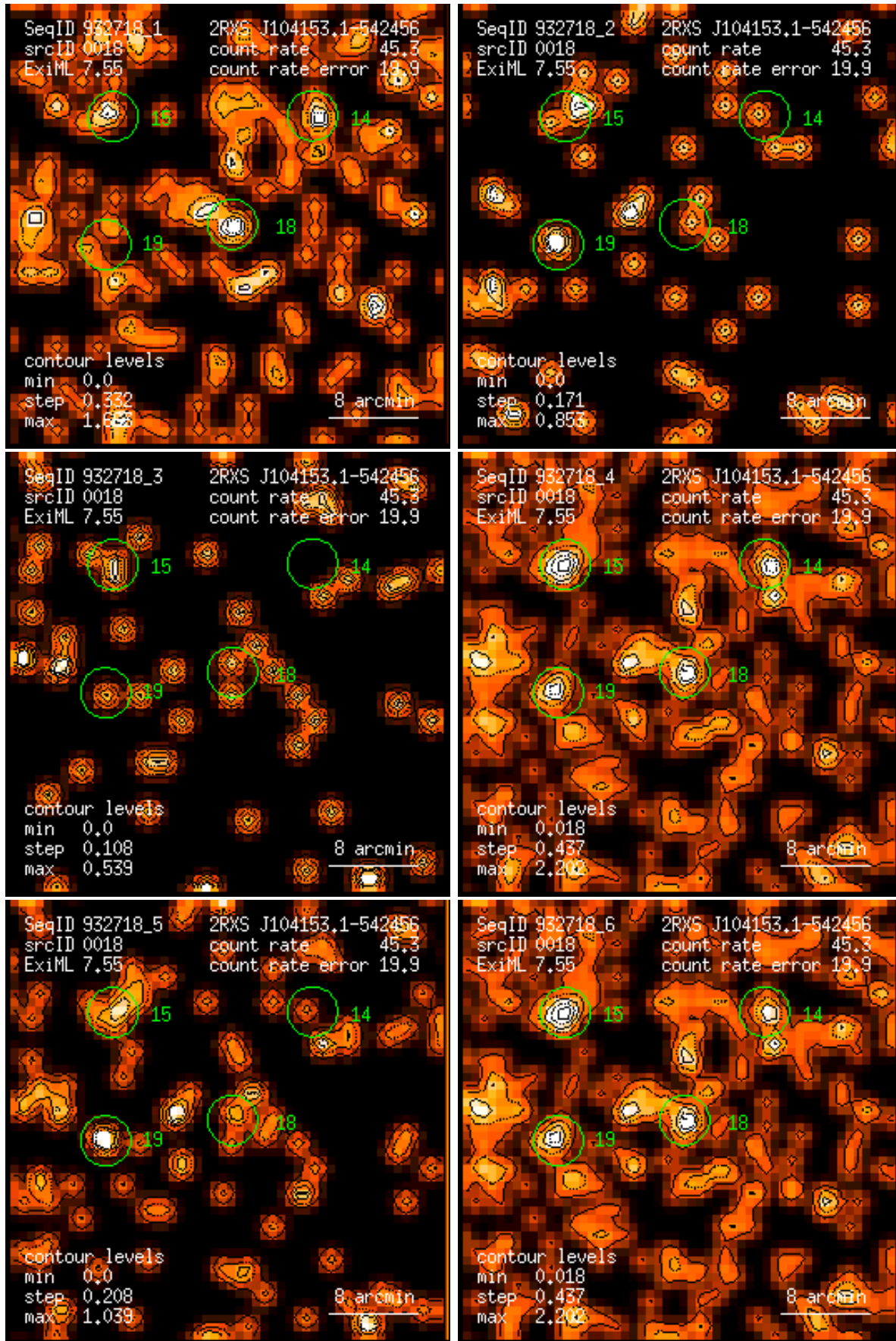
Figure 18: RASS 932718: detection 0018: band rate images, Gaussian filter: (1) PSPC channels 11 – 41, (2) 52 – 90, (3) 91 – 201, (4) 11 – 235, (5) 52 – 201, (6) 11 – 201. Broad band rates in counts/ks. Band rate contour levels in counts/ks/arcmin 2 .
