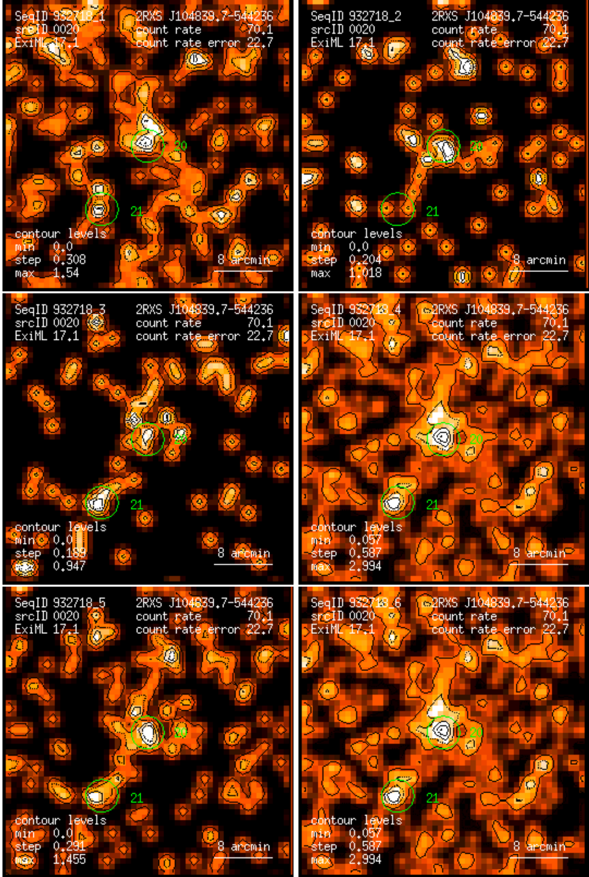
Figure 20: RASS 932718: detection 0020: band rate images, Gaussian filter: (1) PSPC channels 11 – 41, (2) 52 – 90, (3) 91 – 201, (4) 11 – 235, (5) 52 – 201, (6) 11 – 201. Broad band rates in counts/ks. Band rate contour levels in counts/ks/arcmin 2 .
