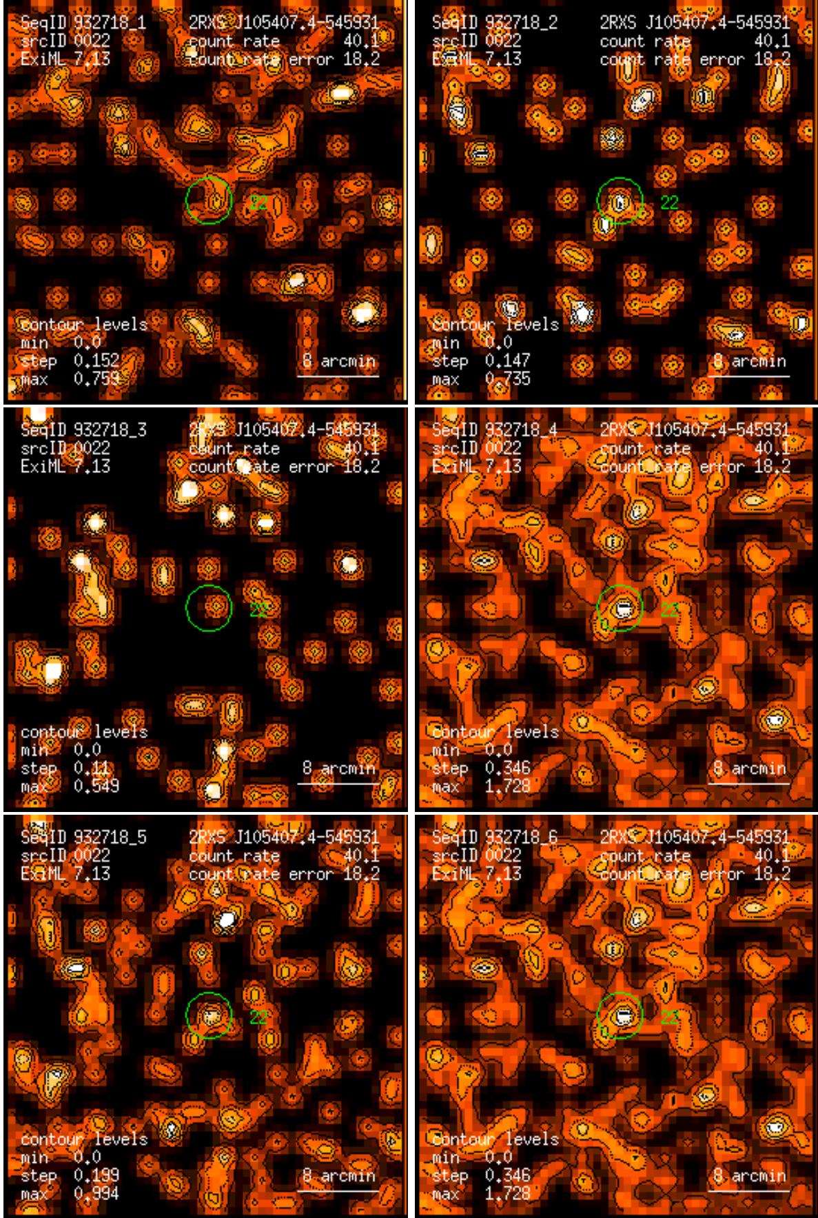
Figure 22: RASS 932718: detection 0022: band rate images, Gaussian filter: (1) PSPC channels 11 – 41, (2) 52 – 90, (3) 91 – 201, (4) 11 – 235, (5) 52 – 201, (6) 11 – 201. Broad band rates in counts/ks. Band rate contour levels in counts/ks/arcmin 2 .
