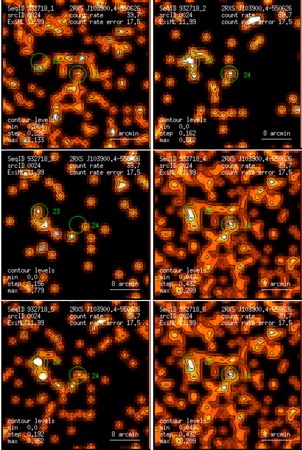
Figure 24: RASS 932718: detection 0024: band rate images, Gaussian filter: (1) PSPC channels 11 – 41, (2) 52 – 90, (3) 91 – 201, (4) 11 – 235, (5) 52 – 201, (6) 11 – 201. Broad band rates in counts/ks. Band rate contour levels in counts/ks/arcmin 2 .
