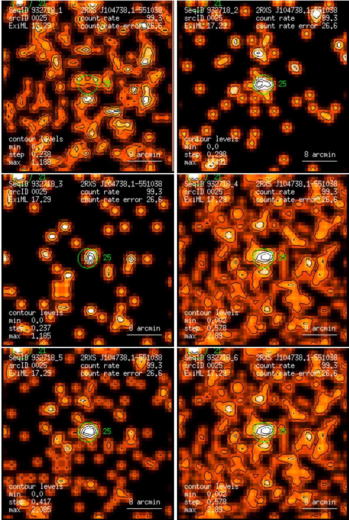
Figure 25: RASS 932718: detection 0025: band rate images, Gaussian filter: (1) PSPC channels 11 – 41, (2) 52 – 90, (3) 91 – 201, (4) 11 – 235, (5) 52 – 201, (6) 11 – 201. Broad band rates in counts/ks. Band rate contour levels in counts/ks/arcmin 2 .
