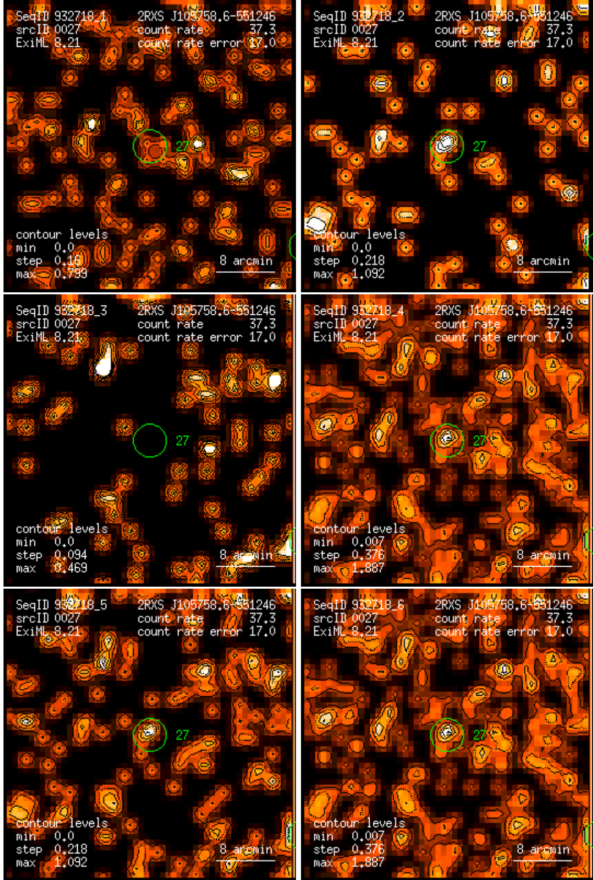
Figure 27: RASS 932718: detection 0027: band rate images, Gaussian filter: (1) PSPC channels 11 – 41, (2) 52 – 90, (3) 91 – 201, (4) 11 – 235, (5) 52 – 201, (6) 11 – 201. Broad band rates in counts/ks. Band rate contour levels in counts/ks/arcmin 2 .
