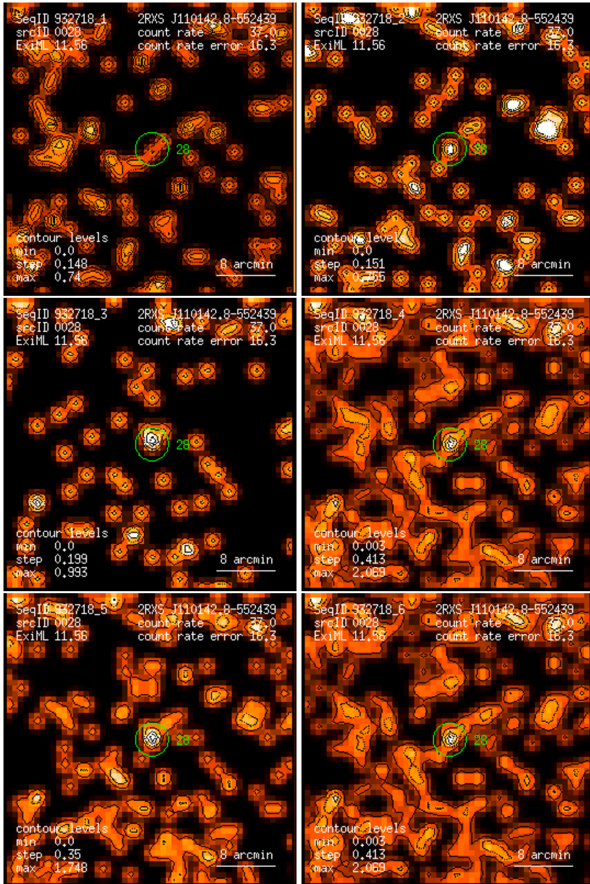
Figure 28: RASS 932718: detection 0028: band rate images, Gaussian filter: (1) PSPC channels 11 – 41, (2) 52 – 90, (3) 91 – 201, (4) 11 – 235, (5) 52 – 201, (6) 11 – 201. Broad band rates in counts/ks. Band rate contour levels in counts/ks/arcmin 2 .
