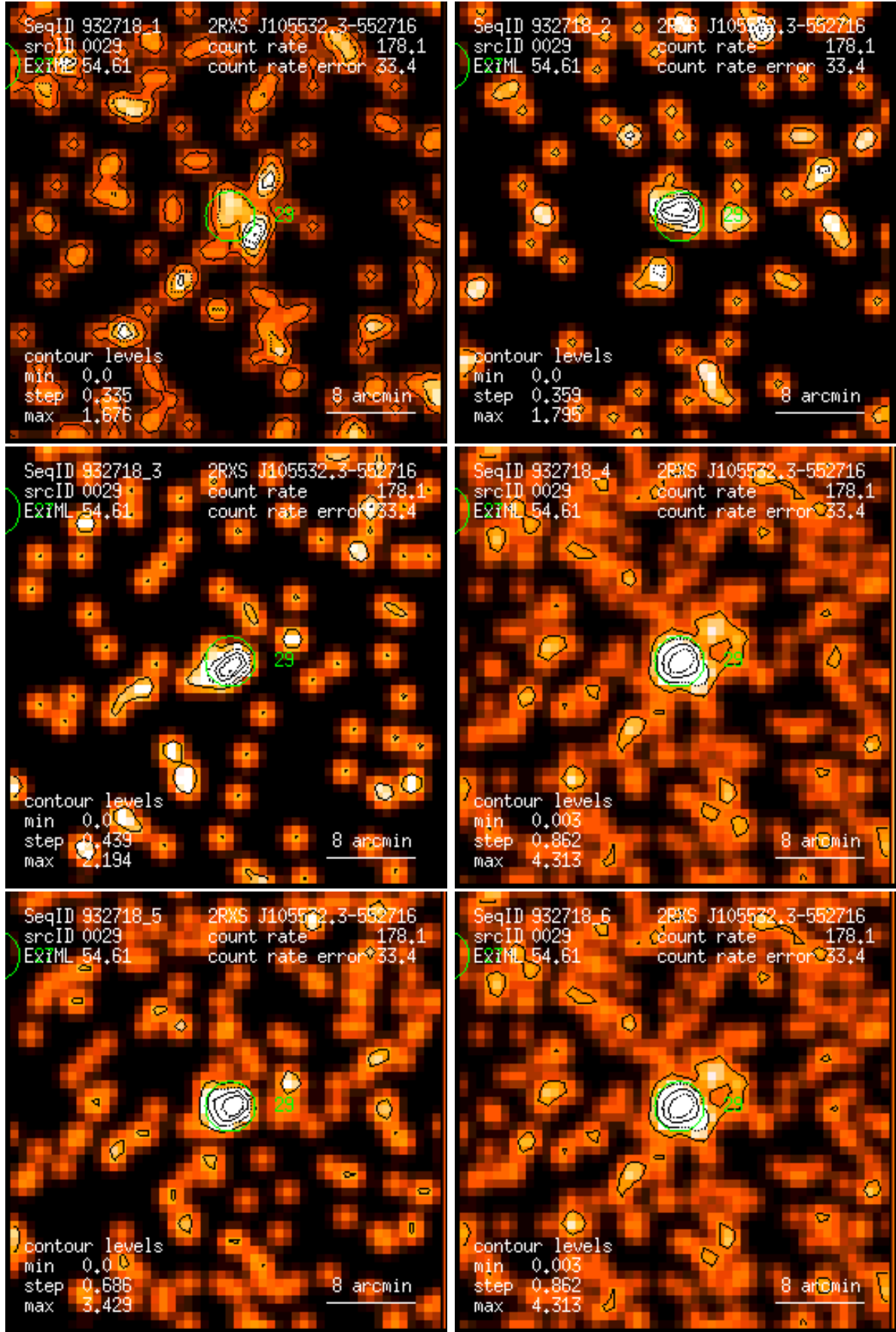
Figure 29: RASS 932718: detection 0029: band rate images, Gaussian filter: (1) PSPC channels 11 – 41, (2) 52 – 90, (3) 91 – 201, (4) 11 – 235, (5) 52 – 201, (6) 11 – 201. Broad band rates in counts/ks. Band rate contour levels in counts/ks/arcmin 2 .
