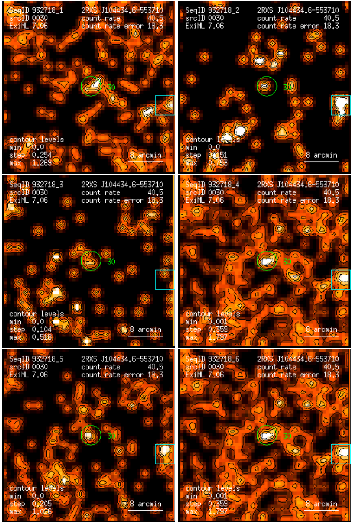
Figure 30: RASS 932718: detection 0030: band rate images, Gaussian filter: (1) PSPC channels 11 – 41, (2) 52 – 90, (3) 91 – 201, (4) 11 – 235, (5) 52 – 201, (6) 11 – 201. Broad band rates in counts/ks. Band rate contour levels in counts/ks/arcmin 2 .
