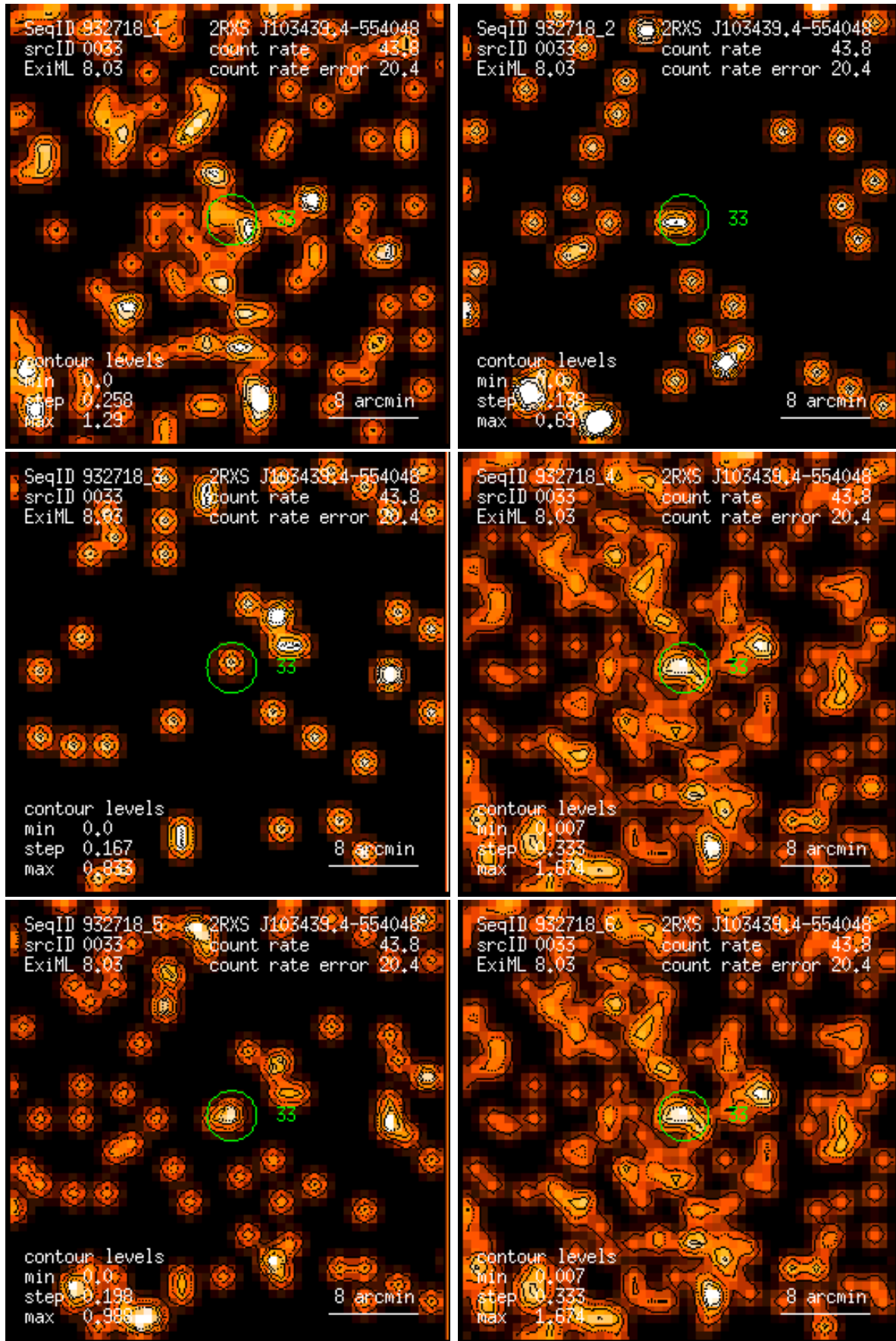
Figure 33: RASS 932718: detection 0033: band rate images, Gaussian filter: (1) PSPC channels 11 – 41, (2) 52 – 90, (3) 91 – 201, (4) 11 – 235, (5) 52 – 201, (6) 11 – 201. Broad band rates in counts/ks. Band rate contour levels in counts/ks/arcmin 2 .
