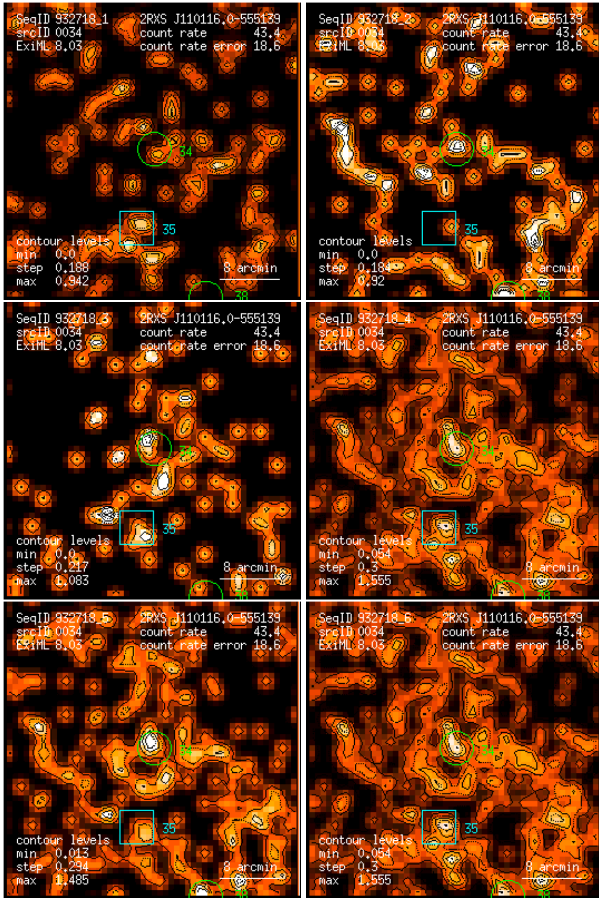
Figure 34: RASS 932718: detection 0034: band rate images, Gaussian filter: (1) PSPC channels 11 – 41, (2) 52 – 90, (3) 91 – 201, (4) 11 – 235, (5) 52 – 201, (6) 11 – 201. Broad band rates in counts/ks. Band rate contour levels in counts/ks/arcmin 2 .
