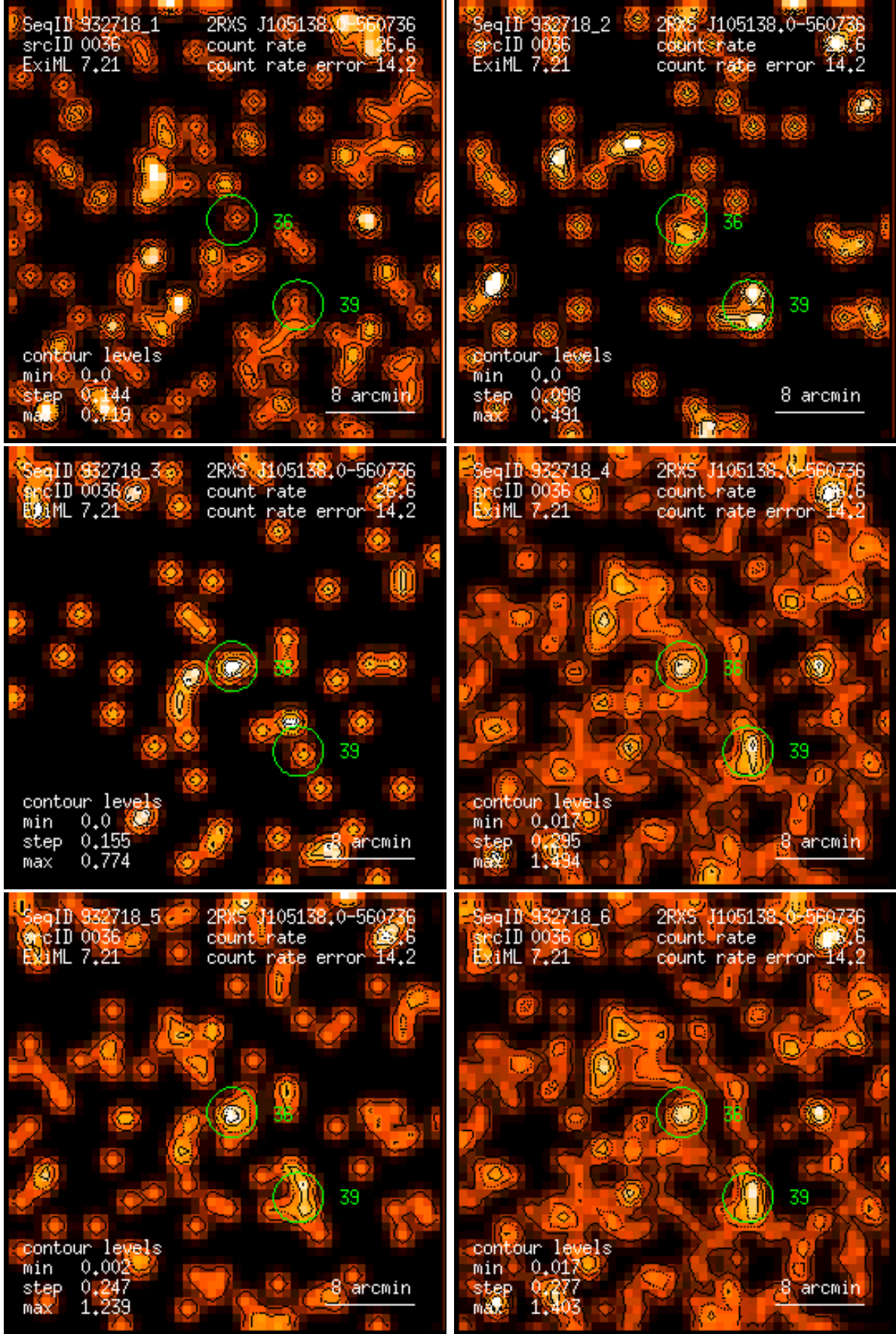
Figure 36: RASS 932718: detection 0036: band rate images, Gaussian filter: (1) PSPC channels 11 – 41, (2) 52 – 90, (3) 91 – 201, (4) 11 – 235, (5) 52 – 201, (6) 11 – 201. Broad band rates in counts/ks. Band rate contour levels in counts/ks/arcmin 2 .
