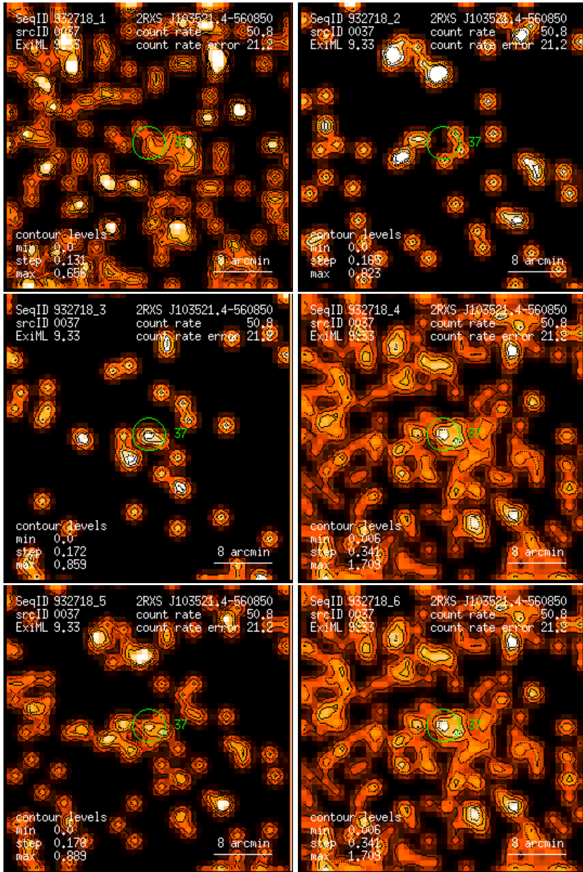
Figure 37: RASS 932718: detection 0037: band rate images, Gaussian filter: (1) PSPC channels 11 – 41, (2) 52 – 90, (3) 91 – 201, (4) 11 – 235, (5) 52 – 201, (6) 11 – 201. Broad band rates in counts/ks. Band rate contour levels in counts/ks/arcmin 2 .
