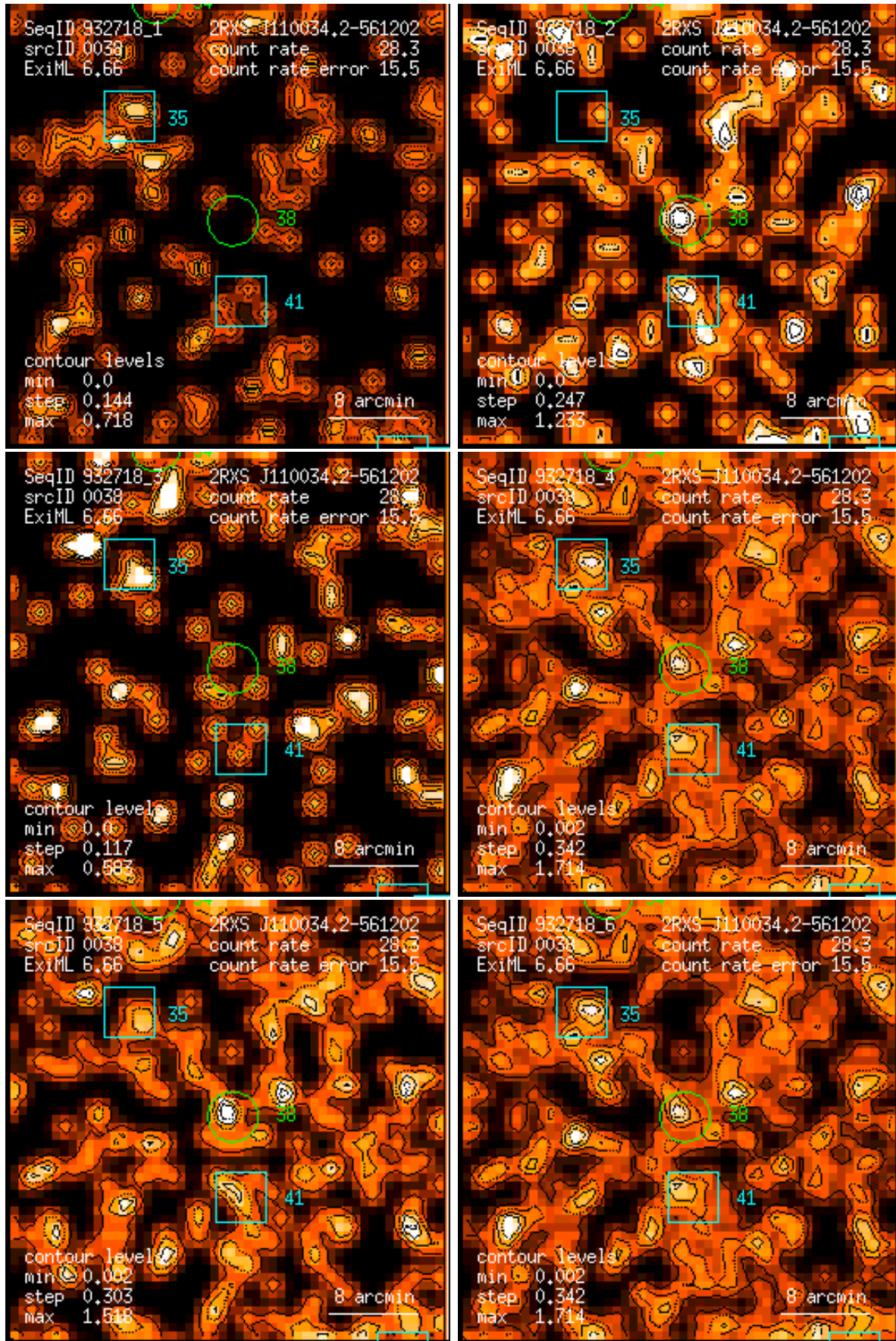
Figure 38: RASS 932718: detection 0038: band rate images, Gaussian filter: (1) PSPC channels 11 – 41, (2) 52 – 90, (3) 91 – 201, (4) 11 – 235, (5) 52 – 201, (6) 11 – 201. Broad band rates in counts/ks. Band rate contour levels in counts/ks/arcmin 2 .
