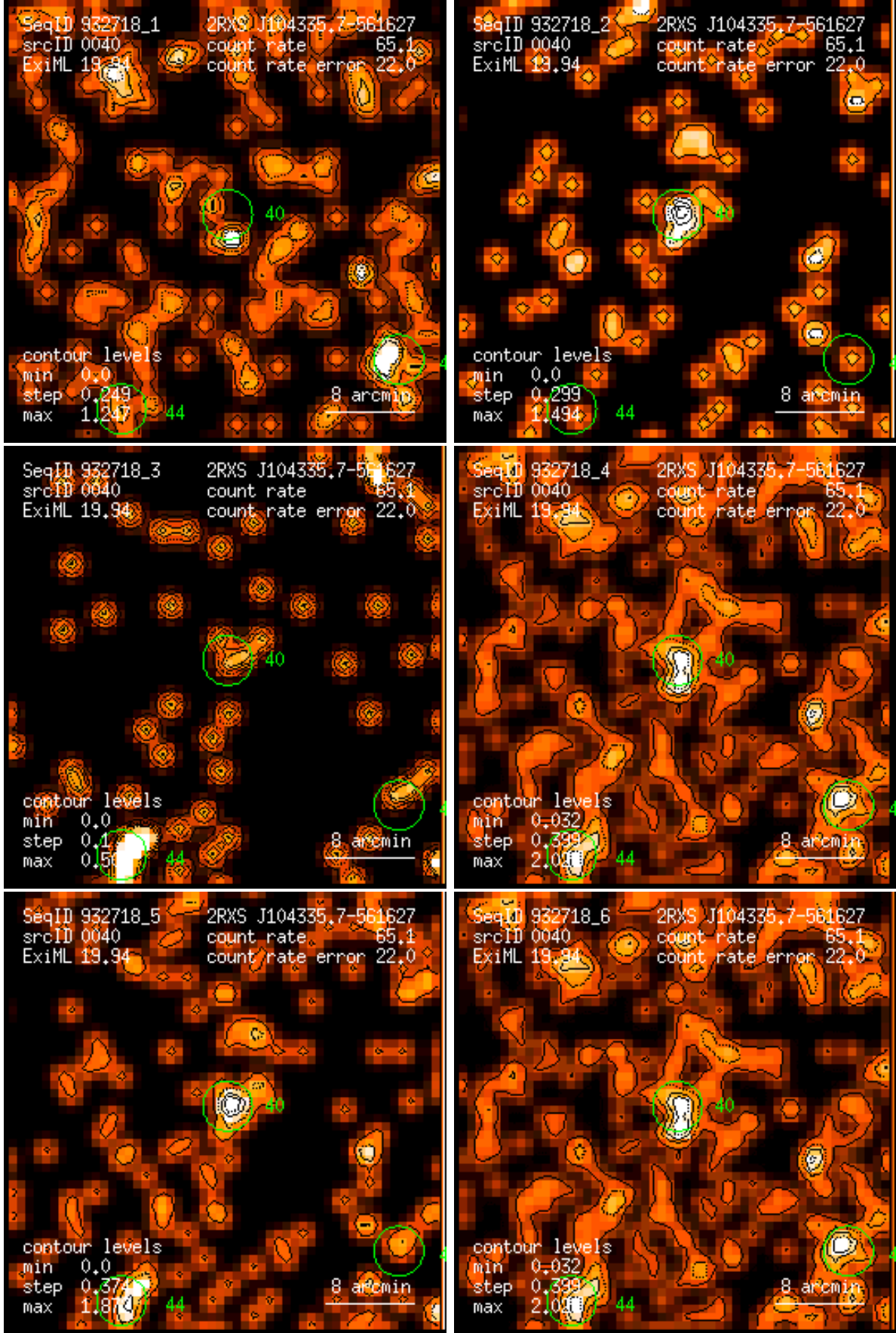
Figure 40: RASS 932718: detection 0040: band rate images, Gaussian filter: (1) PSPC channels 11 – 41, (2) 52 – 90, (3) 91 – 201, (4) 11 – 235, (5) 52 – 201, (6) 11 – 201. Broad band rates in counts/ks. Band rate contour levels in counts/ks/arcmin 2 .
