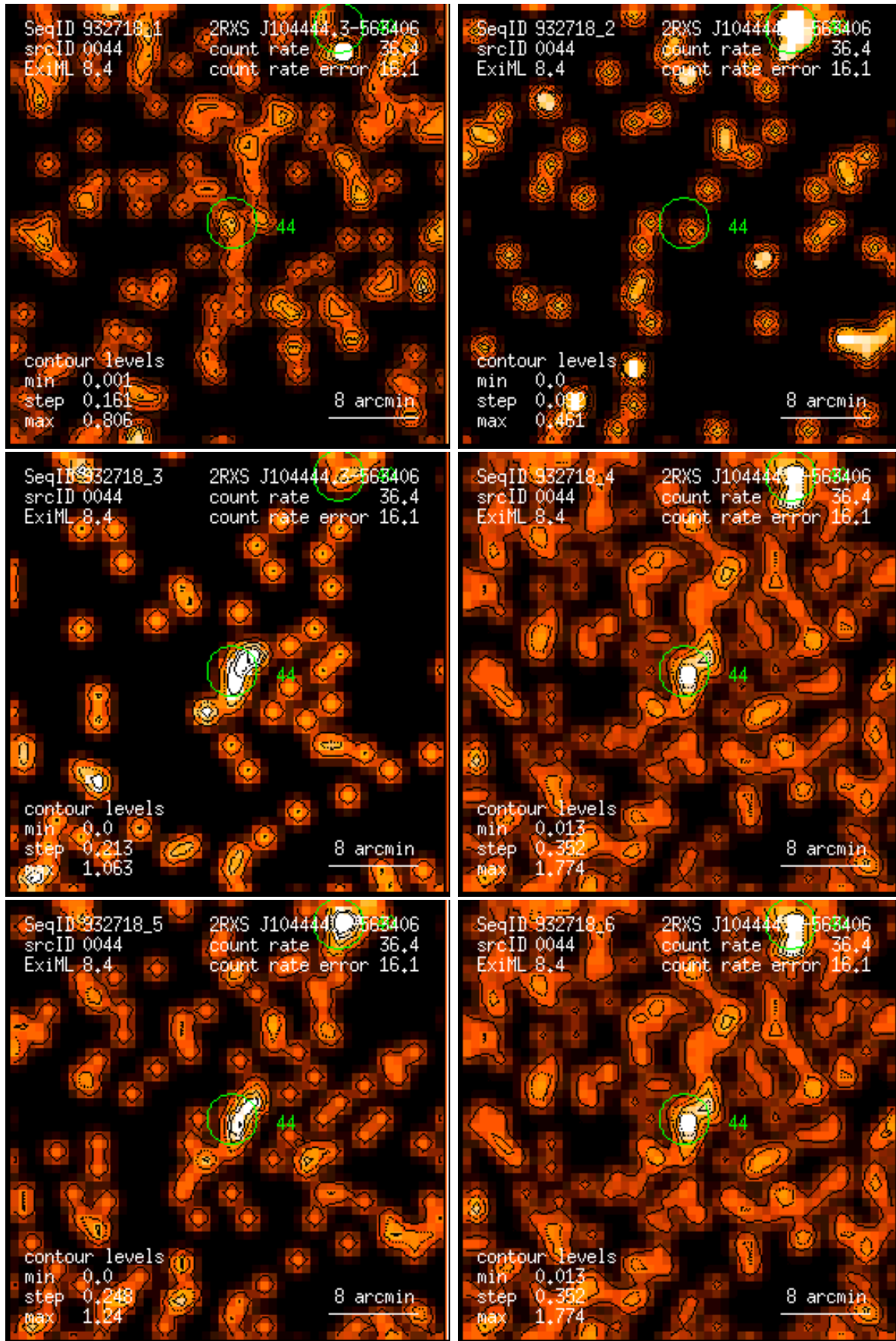
Figure 44: RASS 932718: detection 0044: band rate images, Gaussian filter: (1) PSPC channels 11 – 41, (2) 52 – 90, (3) 91 – 201, (4) 11 – 235, (5) 52 – 201, (6) 11 – 201. Broad band rates in counts/ks. Band rate contour levels in counts/ks/arcmin 2 .
