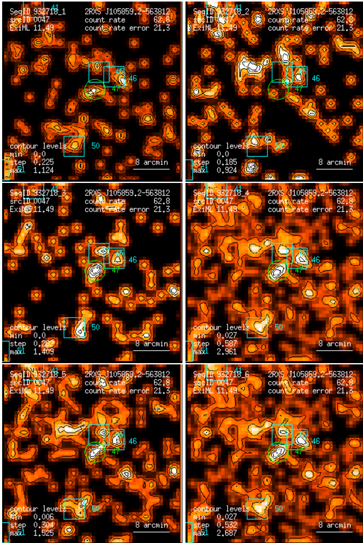
Figure 47: RASS 932718: detection 0047: band rate images, Gaussian filter: (1) PSPC channels 11 – 41, (2) 52 – 90, (3) 91 – 201, (4) 11 – 235, (5) 52 – 201, (6) 11 – 201. Broad band rates in counts/ks. Band rate contour levels in counts/ks/arcmin 2 .
