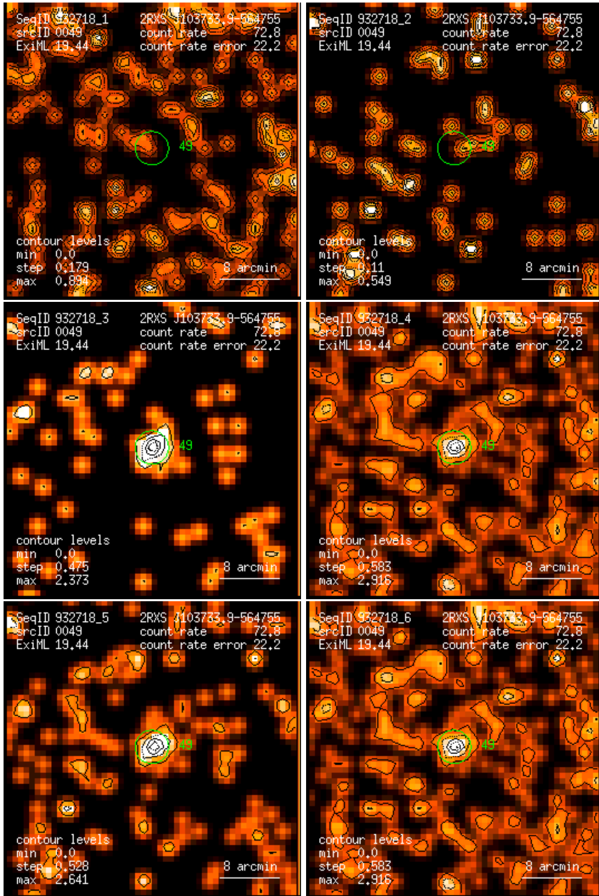
Figure 49: RASS 932718: detection 0049: band rate images, Gaussian filter: (1) PSPC channels 11 – 41, (2) 52 – 90, (3) 91 – 201, (4) 11 – 235, (5) 52 – 201, (6) 11 – 201. Broad band rates in counts/ks. Band rate contour levels in counts/ks/arcmin 2 .
