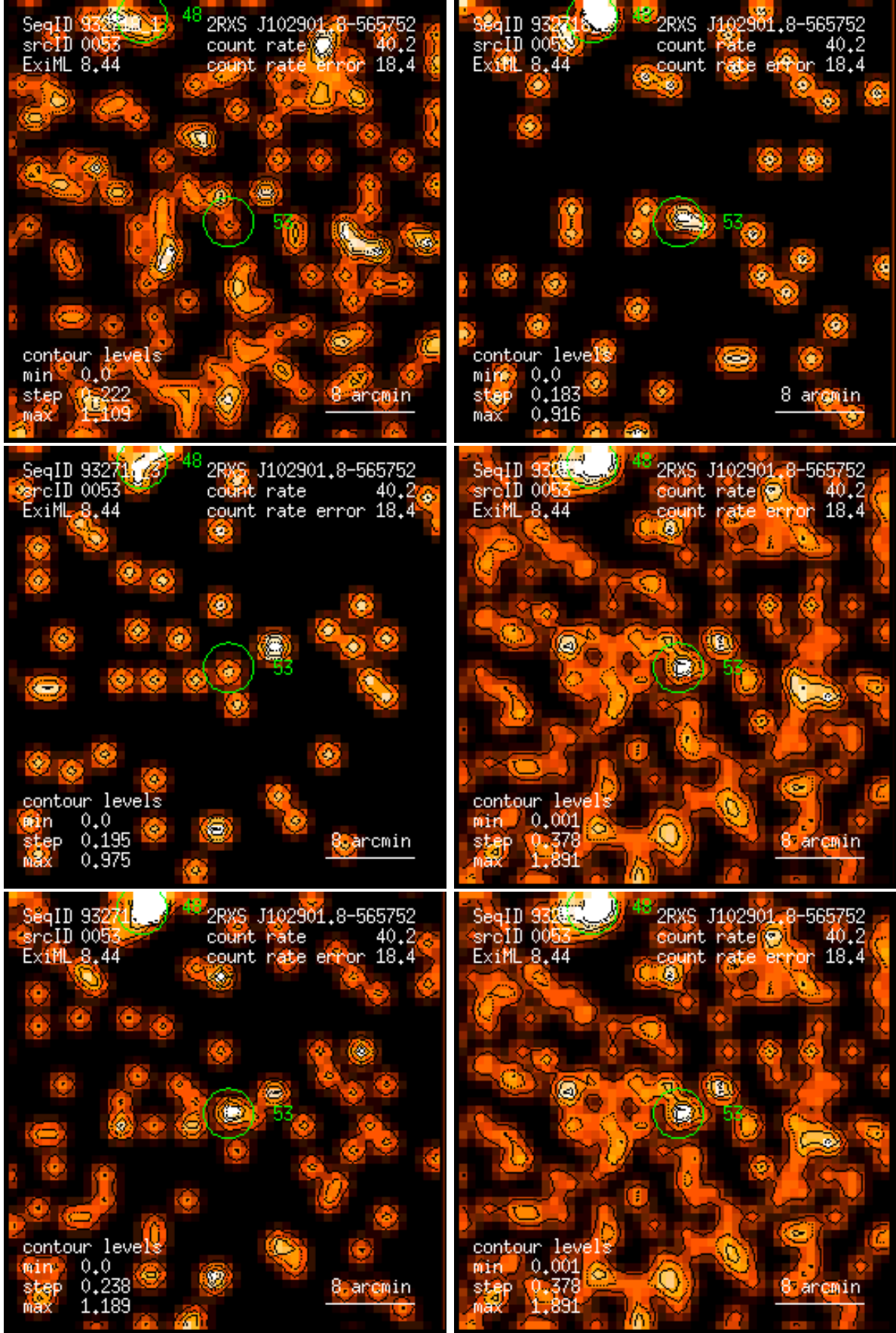
Figure 53: RASS 932718: detection 0053: band rate images, Gaussian filter: (1) PSPC channels 11 – 41, (2) 52 – 90, (3) 91 – 201, (4) 11 – 235, (5) 52 – 201, (6) 11 – 201. Broad band rates in counts/ks. Band rate contour levels in counts/ks/arcmin 2 .
