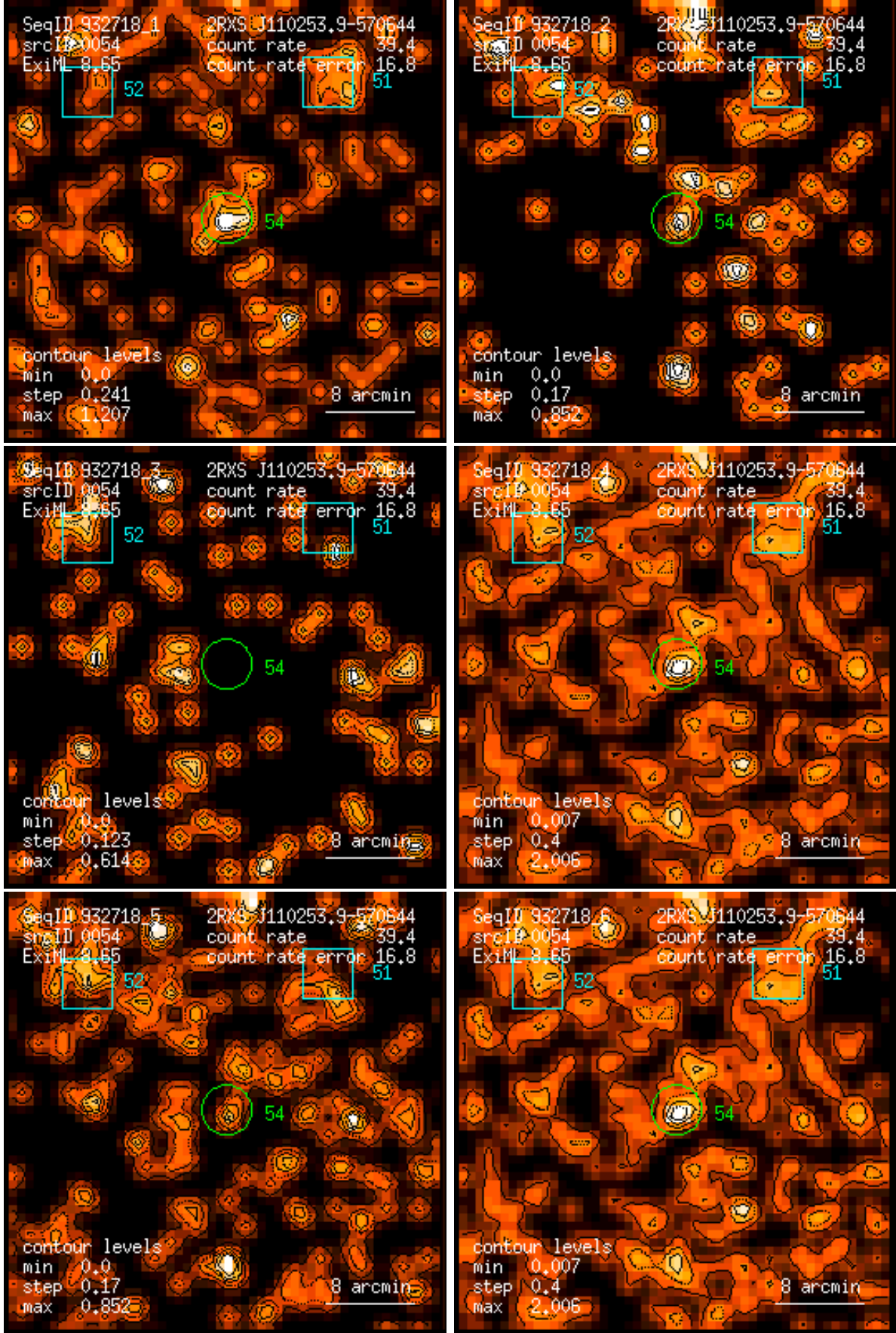
Figure 54: RASS 932718: detection 0054: band rate images, Gaussian filter: (1) PSPC channels 11 – 41, (2) 52 – 90, (3) 91 – 201, (4) 11 – 235, (5) 52 – 201, (6) 11 – 201. Broad band rates in counts/ks. Band rate contour levels in counts/ks/arcmin 2 .
