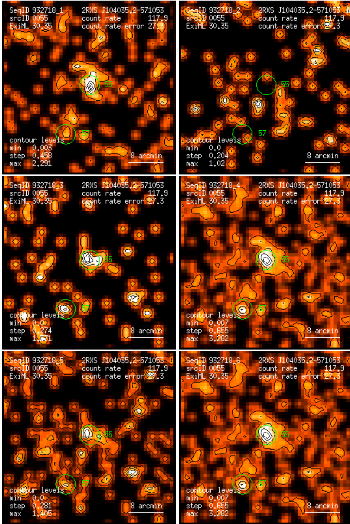
Figure 55: RASS 932718: detection 0055: band rate images, Gaussian filter: (1) PSPC channels 11 – 41, (2) 52 – 90, (3) 91 – 201, (4) 11 – 235, (5) 52 – 201, (6) 11 – 201. Broad band rates in counts/ks. Band rate contour levels in counts/ks/arcmin 2 .
