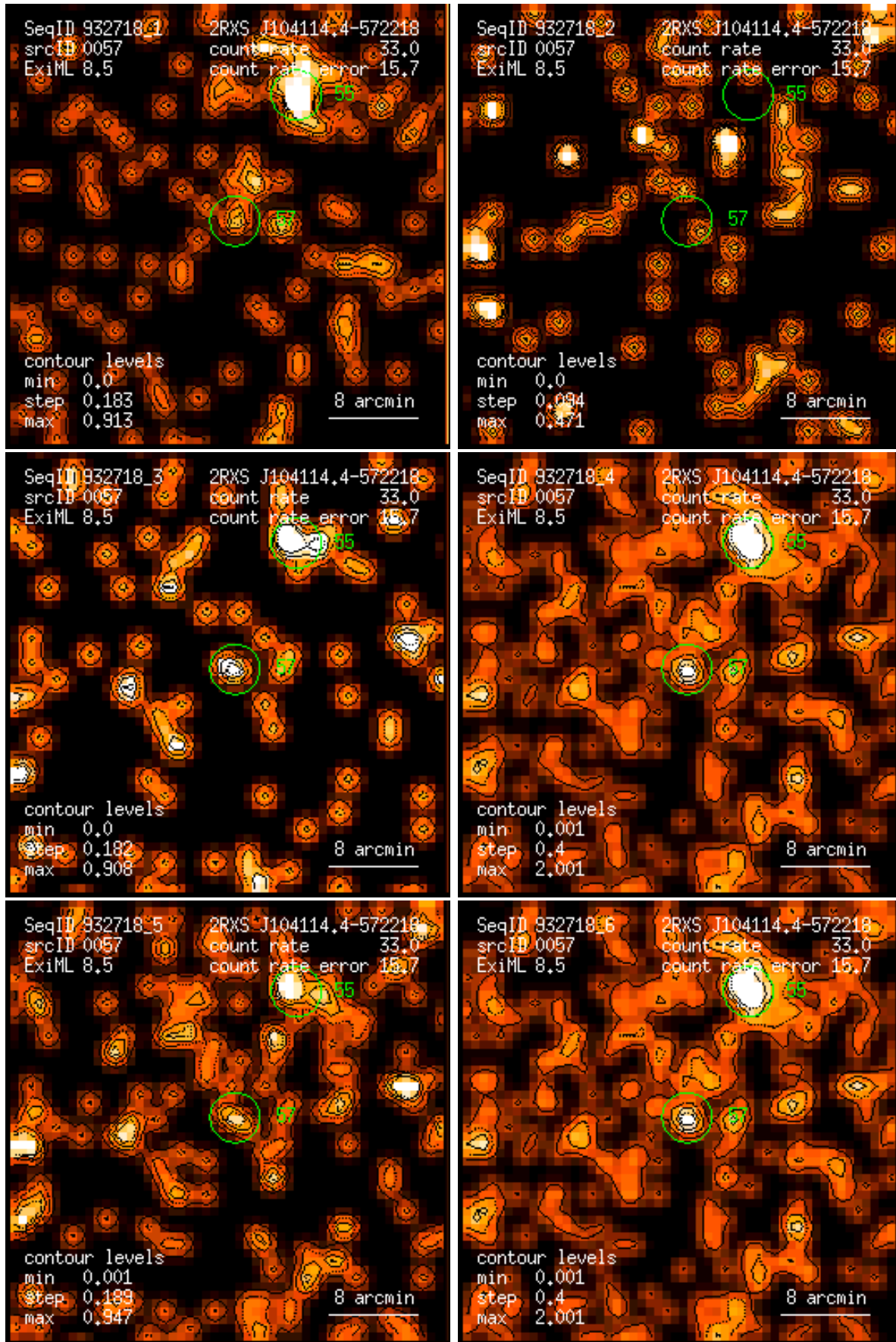
Figure 57: RASS 932718: detection 0057: band rate images, Gaussian filter: (1) PSPC channels 11 – 41, (2) 52 – 90, (3) 91 – 201, (4) 11 – 235, (5) 52 – 201, (6) 11 – 201. Broad band rates in counts/ks. Band rate contour levels in counts/ks/arcmin 2 .
