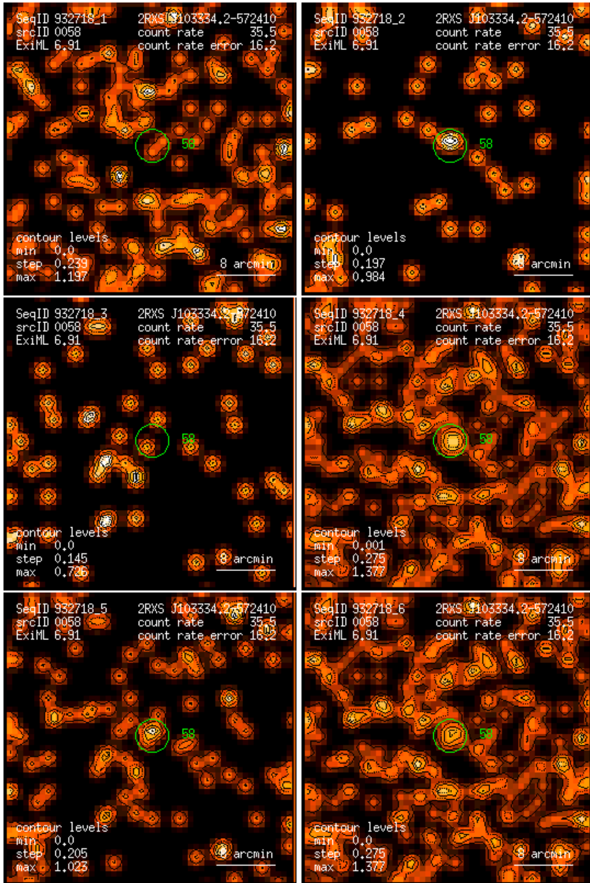
Figure 58: RASS 932718: detection 0058: band rate images, Gaussian filter: (1) PSPC channels 11 – 41, (2) 52 – 90, (3) 91 – 201, (4) 11 – 235, (5) 52 – 201, (6) 11 – 201. Broad band rates in counts/ks. Band rate contour levels in counts/ks/arcmin 2 .
