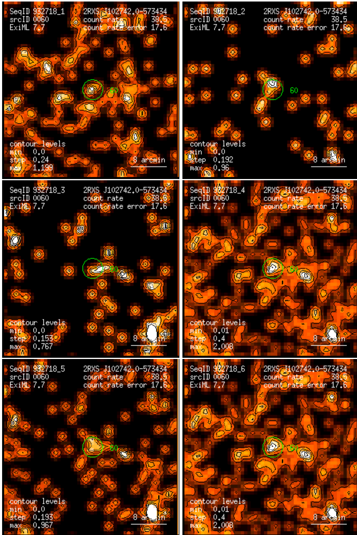
Figure 60: RASS 932718: detection 0060: band rate images, Gaussian filter: (1) PSPC channels 11 – 41, (2) 52 – 90, (3) 91 – 201, (4) 11 – 235, (5) 52 – 201, (6) 11 – 201. Broad band rates in counts/ks. Band rate contour levels in counts/ks/arcmin 2 .
